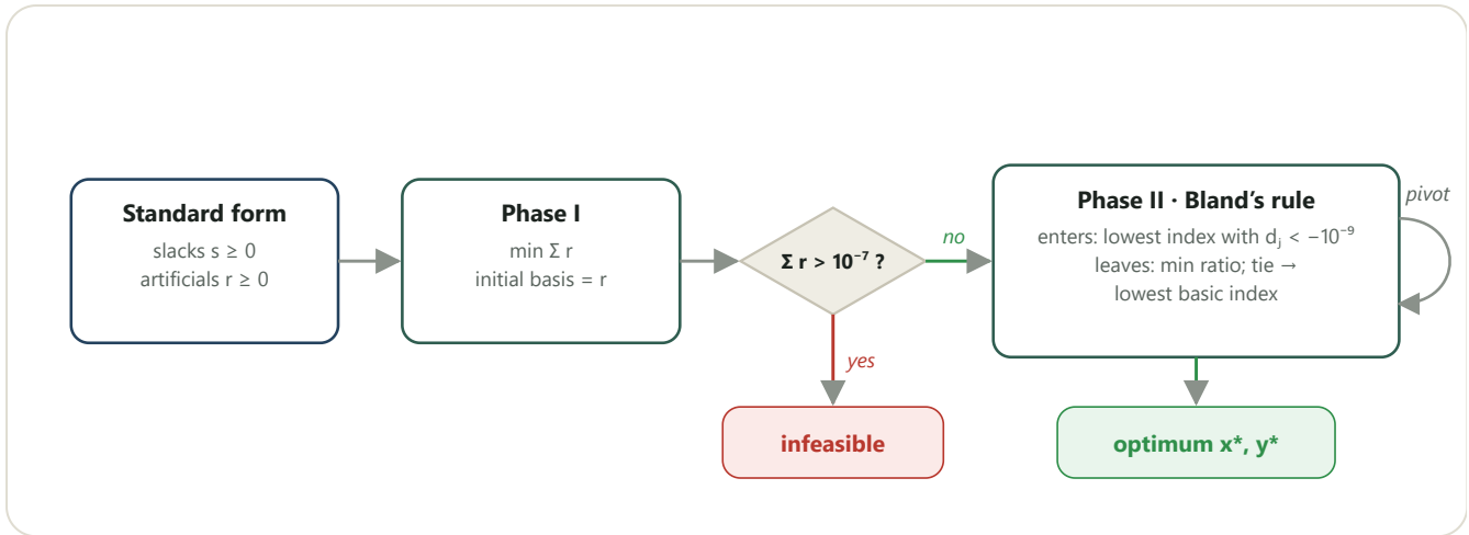
FIGURE 3 Two-phase simplex flow. Tolerances are those in the RatioAvis 1.1.0 source code.
