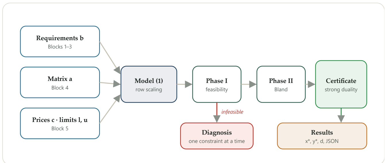
FIGURE 1 Solver architecture. Data from blocks 1–5 build the model; phase I seeks feasibility, phase II the optimum, and the duality certificate validates the solution before it is shown. If there is no solution, a diagnosis identifies the conflicting constraint.
