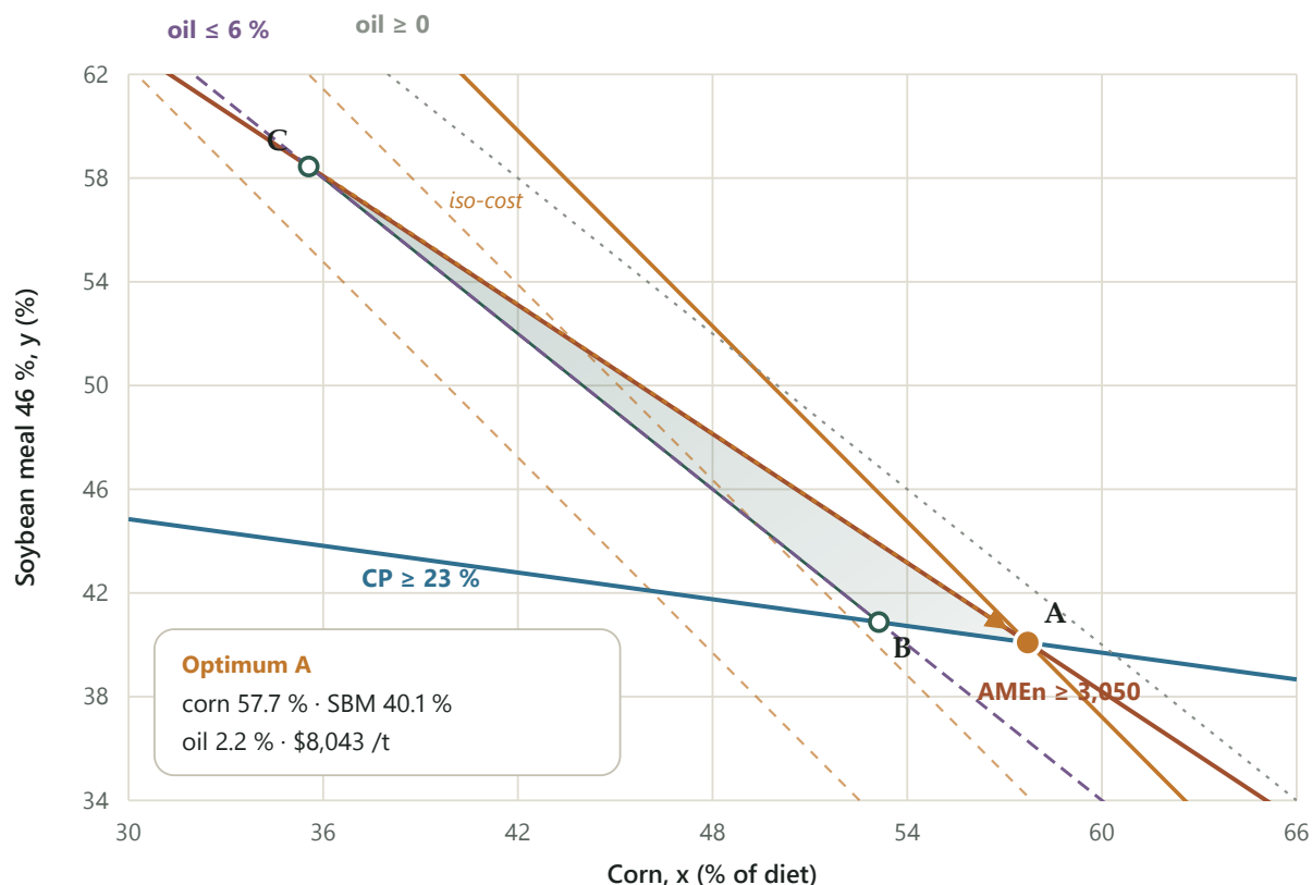
FIGURE 2 Feasible region of a reduced teaching model. Corn ( x ) and soybean meal 46 % ( y ); oil = 100 - x - y , at most 6 %. Requirements: protein \geq 23 % and AMEn \geq 3,050 kcal/kg, using the app's matrix and prices. Simplex moves from vertex to vertex until A , where energy and protein cross: 57.7 % corn, 40.1 % soybean meal and 2.2 % oil. It is an illustration; the real case has 14 variables and 39 constraints.
