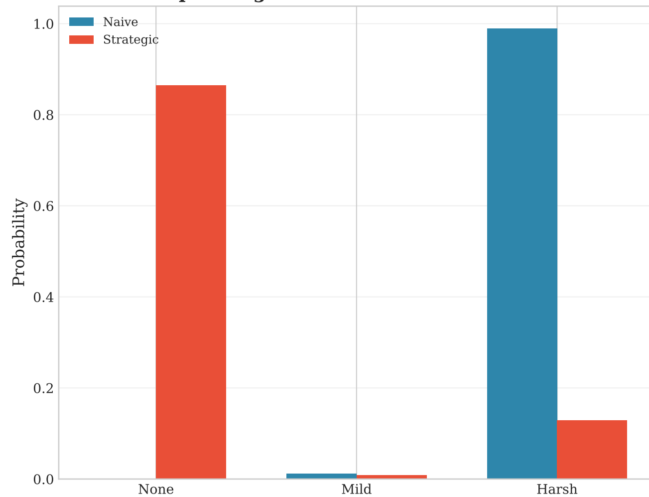
Exp 2: Dog Whistle Action Distribution
