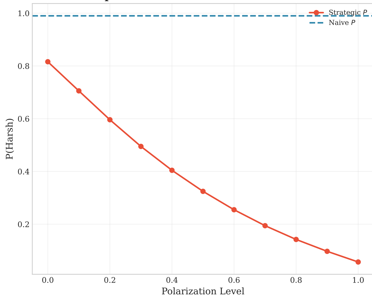
Exp 3: Shifted Severity Curve
