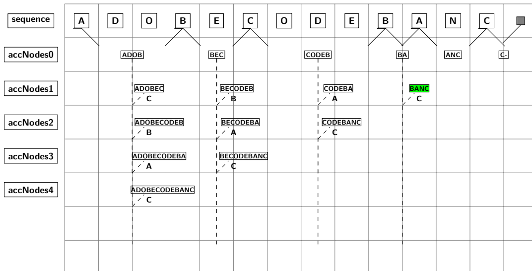
Figure 1: Search for minimum substring example.
