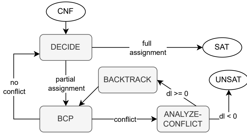
Fig. 15: The DPLL algorithm for SAT solving.
