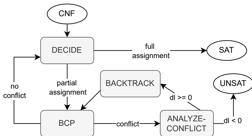
Fig. 12: The DPLL algorithm for SAT solving.
