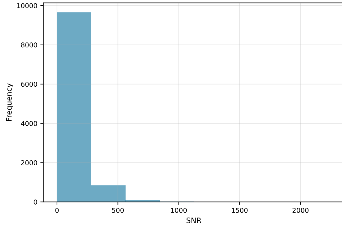
SNR Distribution
