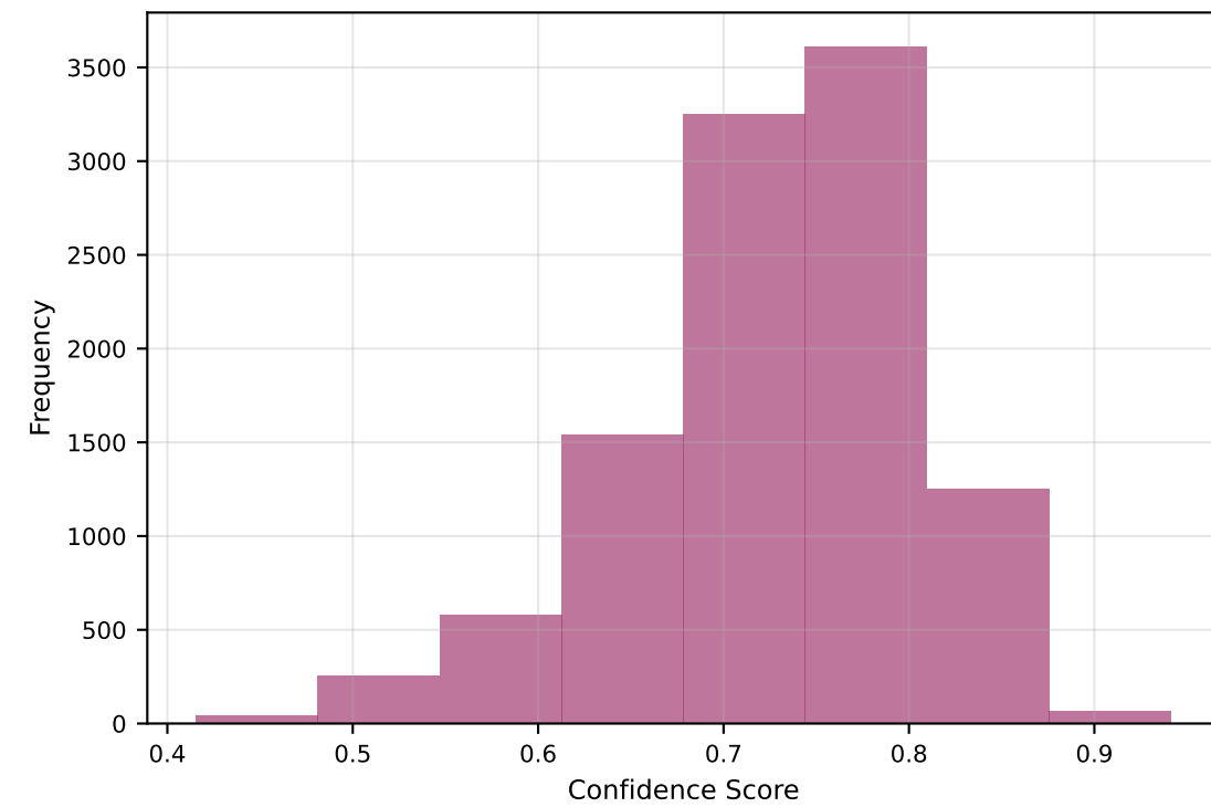
Confidence Distribution
