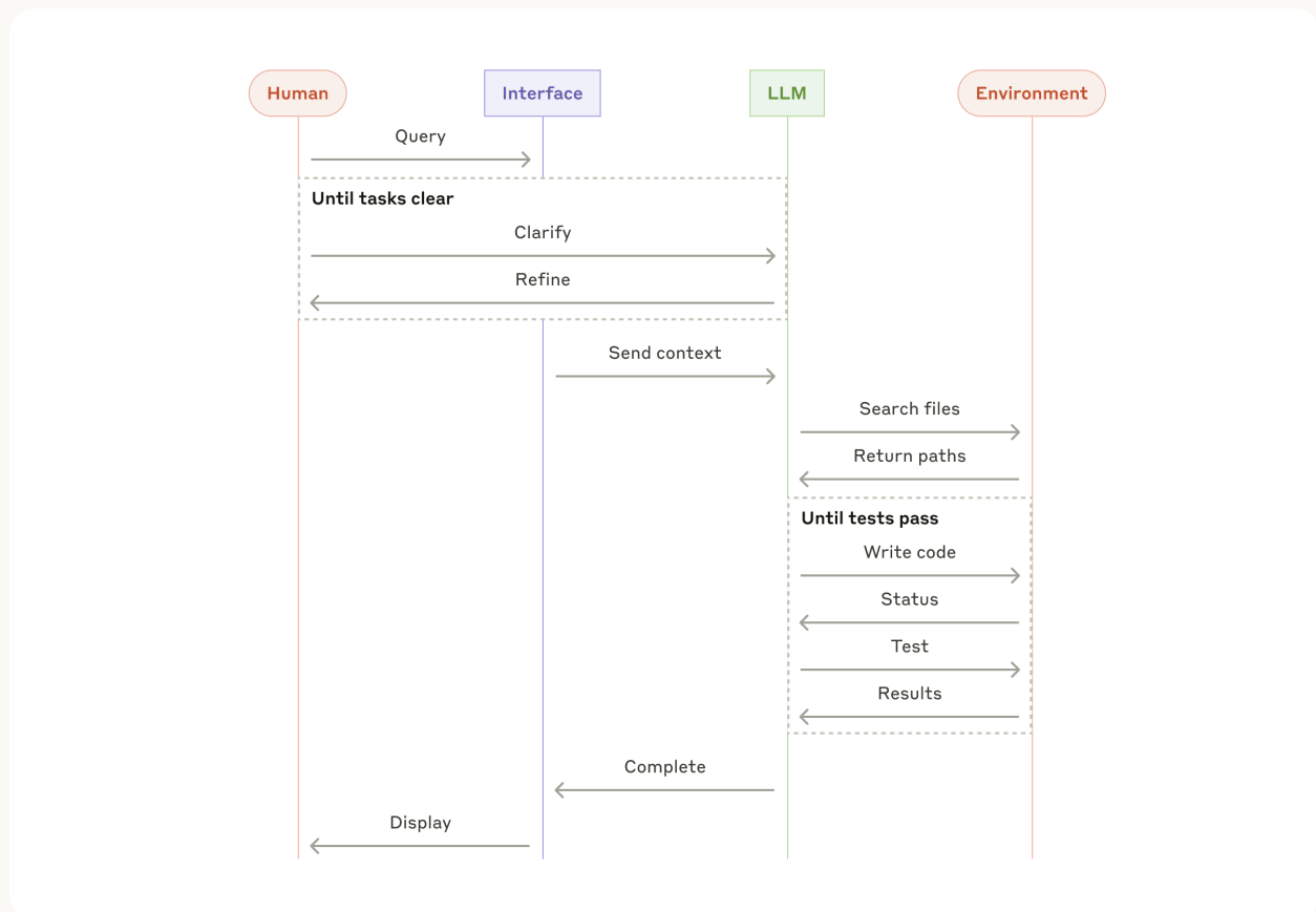
High-level flow of a coding agent
