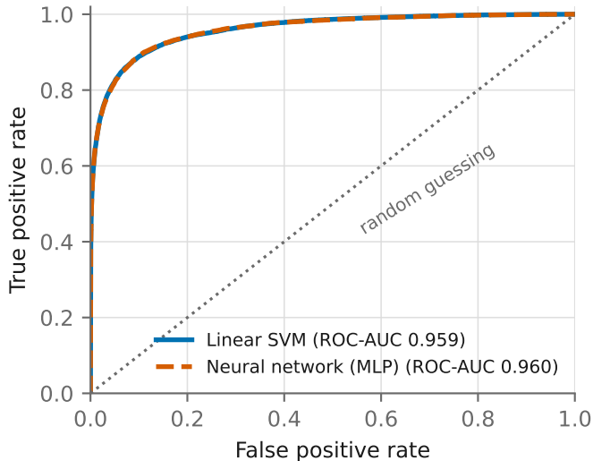
Dataset B: Wikipedia (toxicity)
