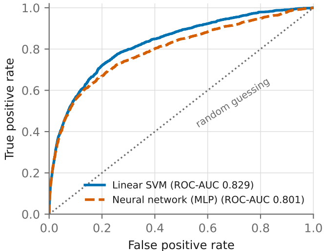
Dataset A: Davidson (hate speech)
