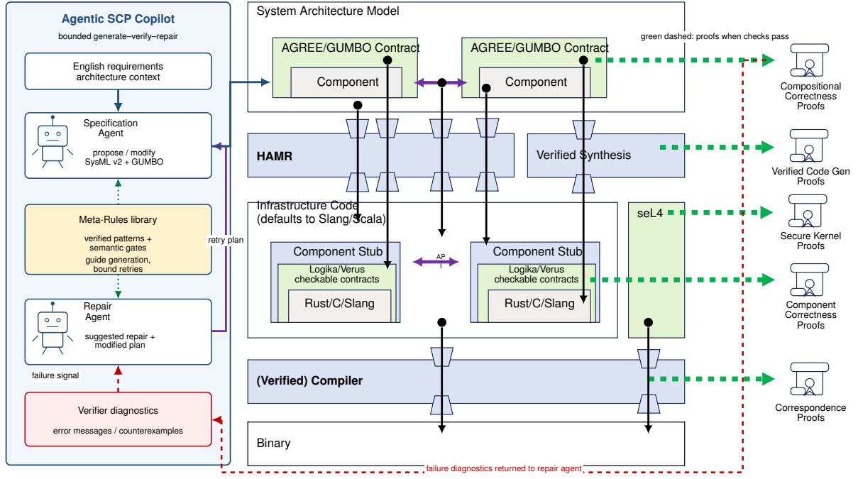
Fig. 1. Agentic SCP/INSPECTA workflow integrating the high-assurance development layers with a Meta-Rule-guided generate–verify–repair loop. Green dashed arrows denote successful proof artifacts; the red dashed arrow denotes verifier-failure diagnostics returned to the repair agent for a bounded retry.
