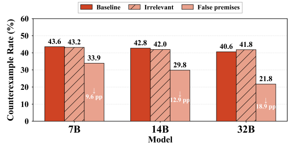
Figure 2: False premises reduce verifier counterexample coverage. Across model scales, the false-premise condition produces substantially fewer counterexample tests than both the baseline and irrelevant-control.
