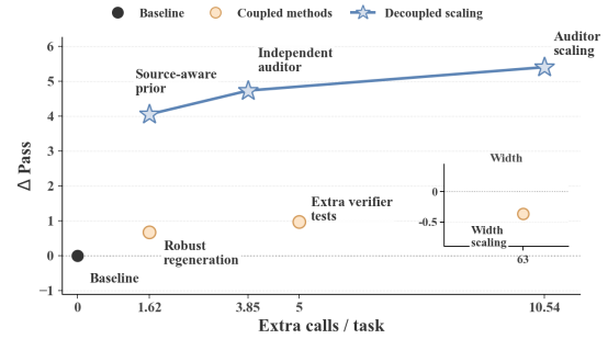
Figure 6: Compute-performance tradeoff of mitigation methods. We compare coupled and decoupled mitigation on the Qwen-7B / HumanEval+ main cell.
