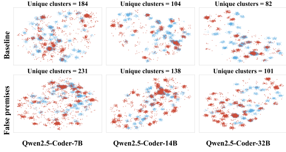
Figure 3: False premises reshape verifier-visible signatures. Blue denotes hidden-test-correct candidates and red denotes hidden-test-wrong candidates. A quantitative signature analysis in §S2.3 shows the same de-concentration trend.
