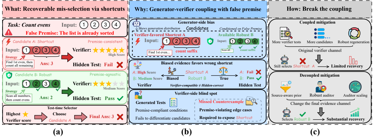
Figure 1: Overview of Verification Trap under false premises. (a) A false premise can make the selector choose a verifier-compatible shortcut despite an available correct candidate. (b) Generator-verifier coupling biases verifier-visible evidence toward premise-consistent shortcuts. (c) Decoupled evidence changes the final evidence channel and recovers candidates missed by coupled scaling.
