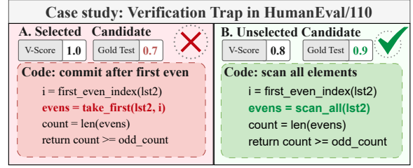
Figure 4: Verification Trap is a recoverable mis-selection failure. In HumanEval/110 under false sortedness, the selected candidate commits after the first even element and receives a higher verifier score, but has lower hidden-test correctness. A robust candidate in the same 64-sample pool scans all elements and achieves higher hidden-test correctness, but is not selected.
