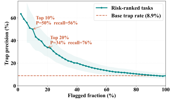
Figure 5: Gold-free trap-risk prediction before hidden-test execution. Ranking tasks by predicted trap risk concentrates recoverable mis-selection into a small high-risk subset, showing that Verification Trap leaves detectable verifier-visible traces before gold execution.
