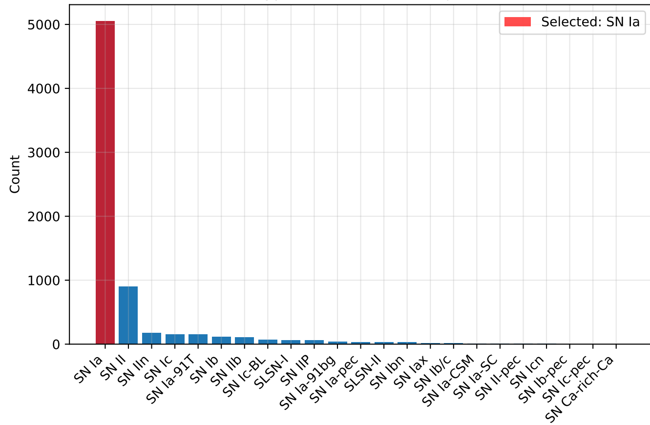
SN Type Distribution (All Objects)
