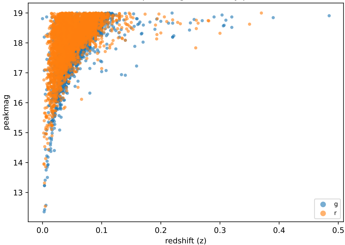
redshift vs peakmag (colored by peakfilt)
