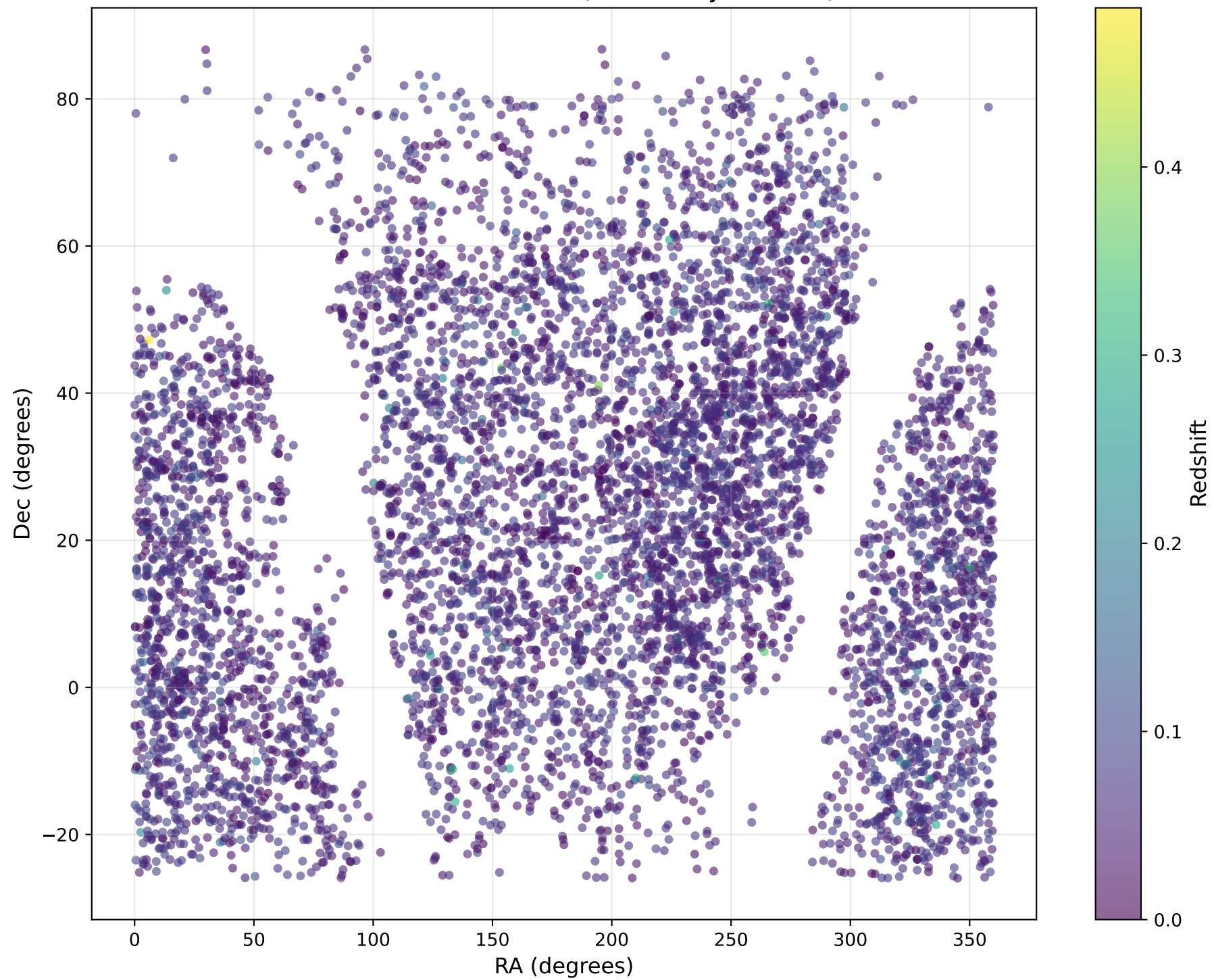
RA vs Dec Scatter Plot (colored by redshift)
