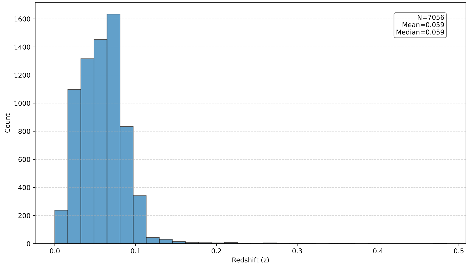
Distribution of Redshift
