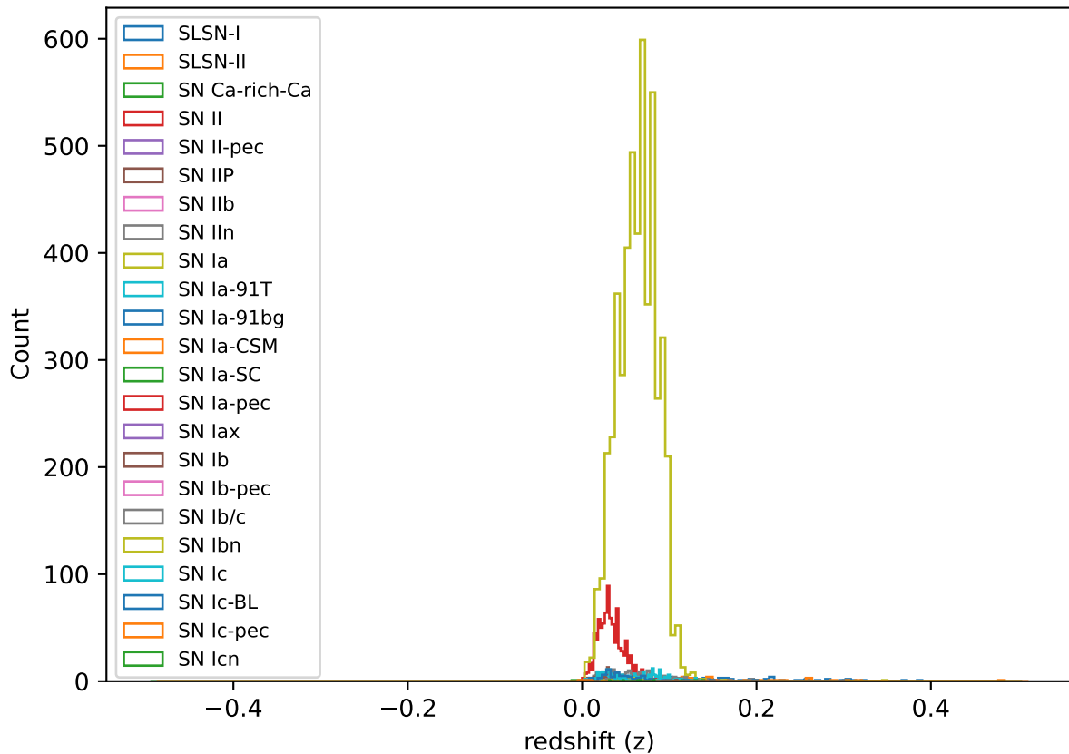
Redshift distribution by type
