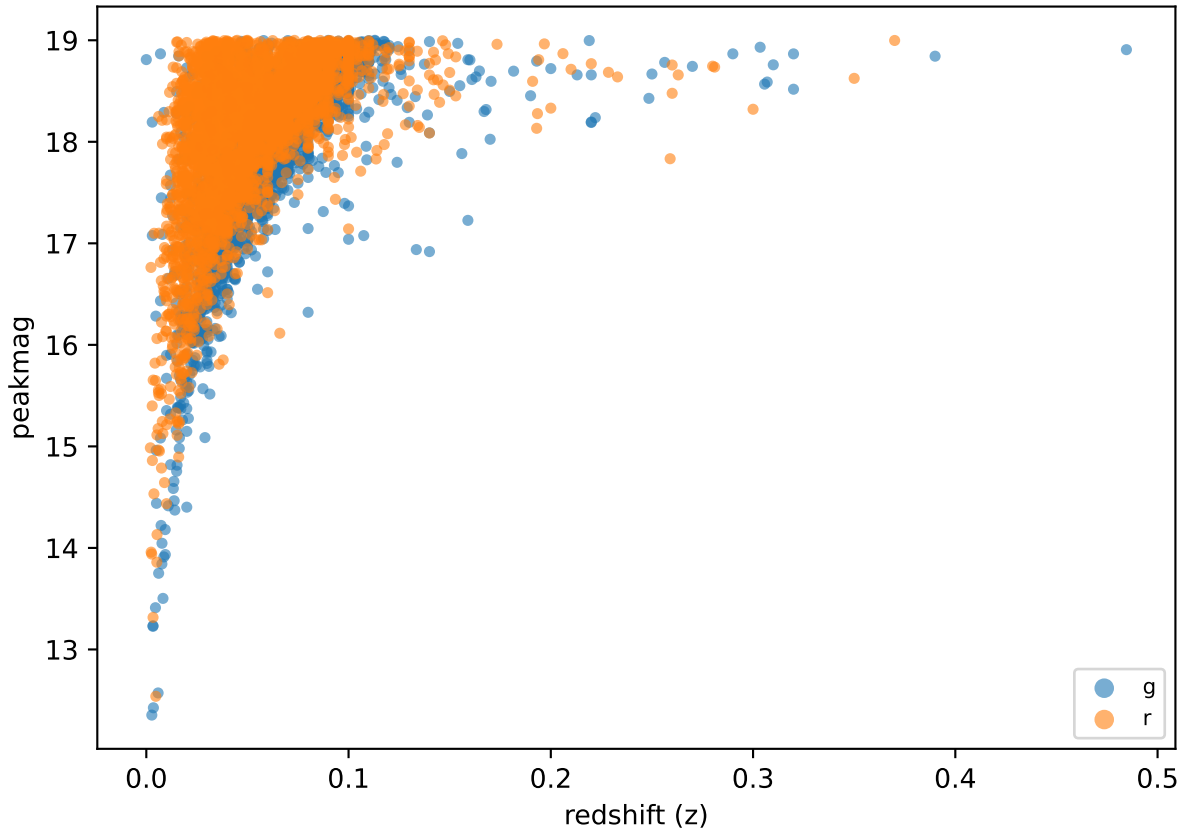
redshift vs peakmag (colored by peakfilt)
