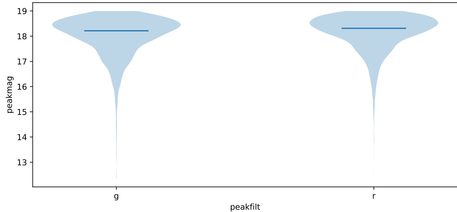
Peak magnitude by filter (violin)
