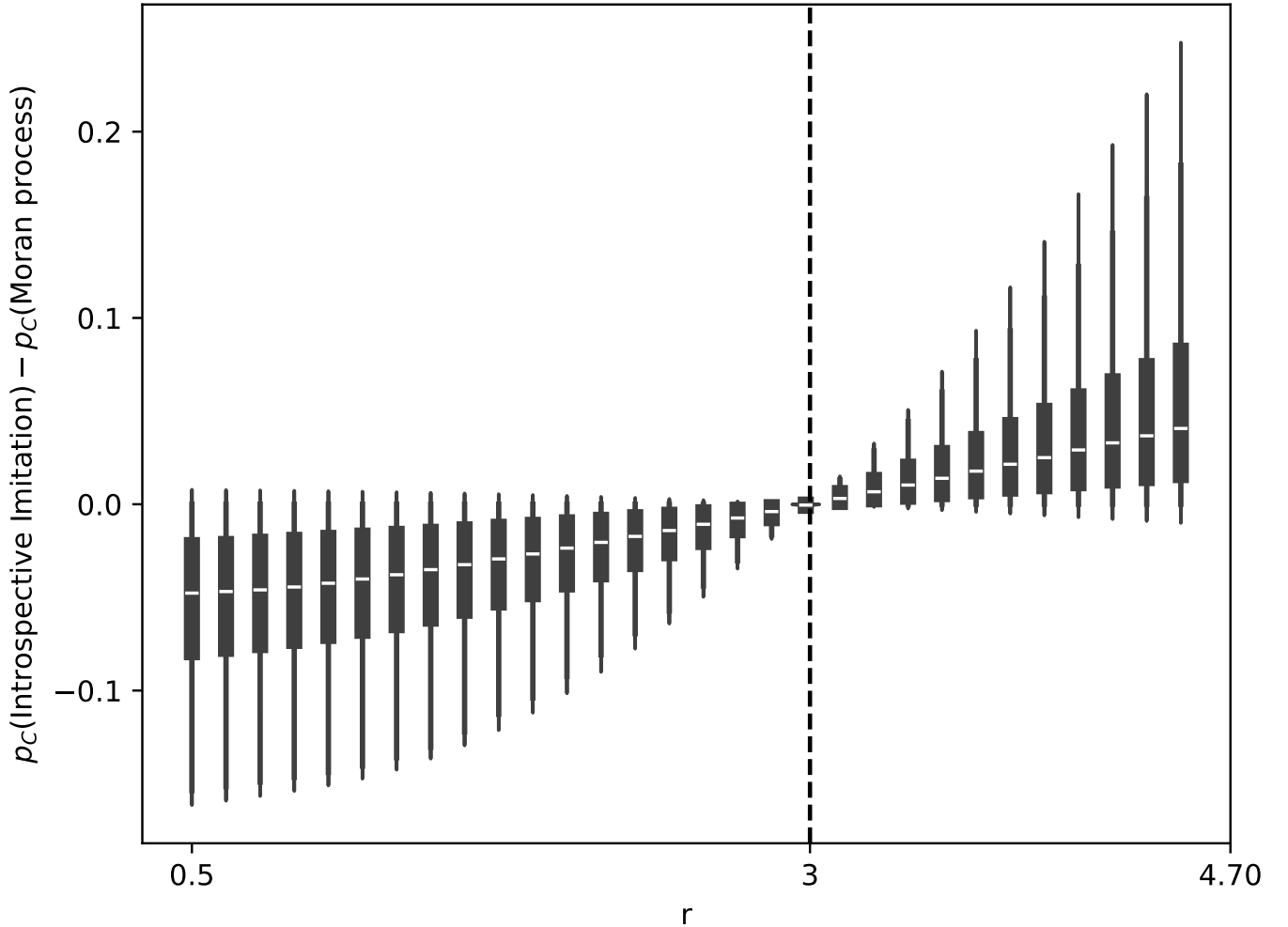
Figure 9: p_C(\text{IID}) - p_C(\text{Moran}) as a function of r for N = 3 (linear population). The dashed vertical line marks r = N = 3 . The IQR collapses to near zero at the threshold before expanding for r > N .
