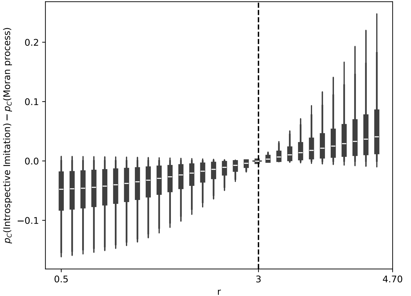
Figure 8: Comparison of p_C under the Moran process and Introspective Imitation Dynamics for N = 3 .
