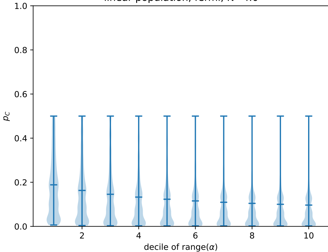
linear population, fermi, N=4.0
