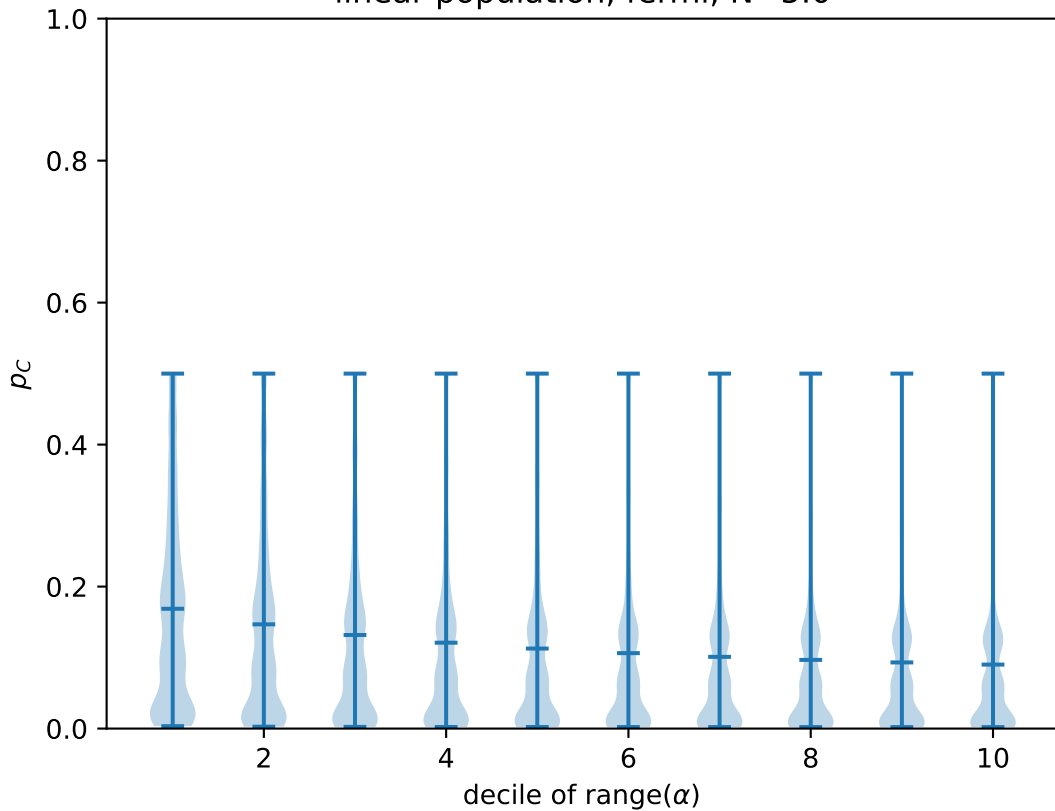
linear population, fermi, N=5.0
