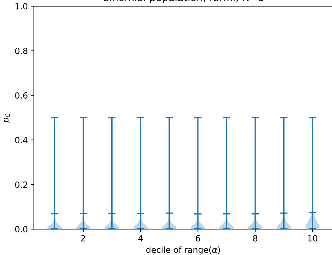
binomial population, fermi, N=5
