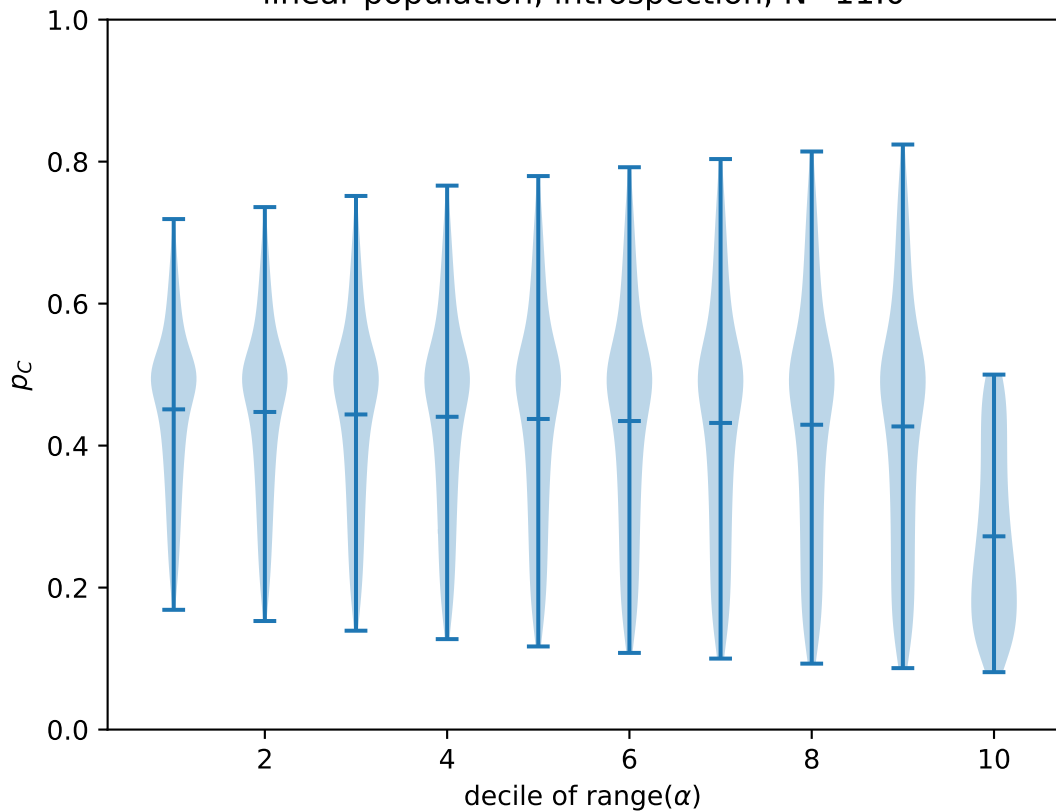
linear population, introspection, N=11.0
