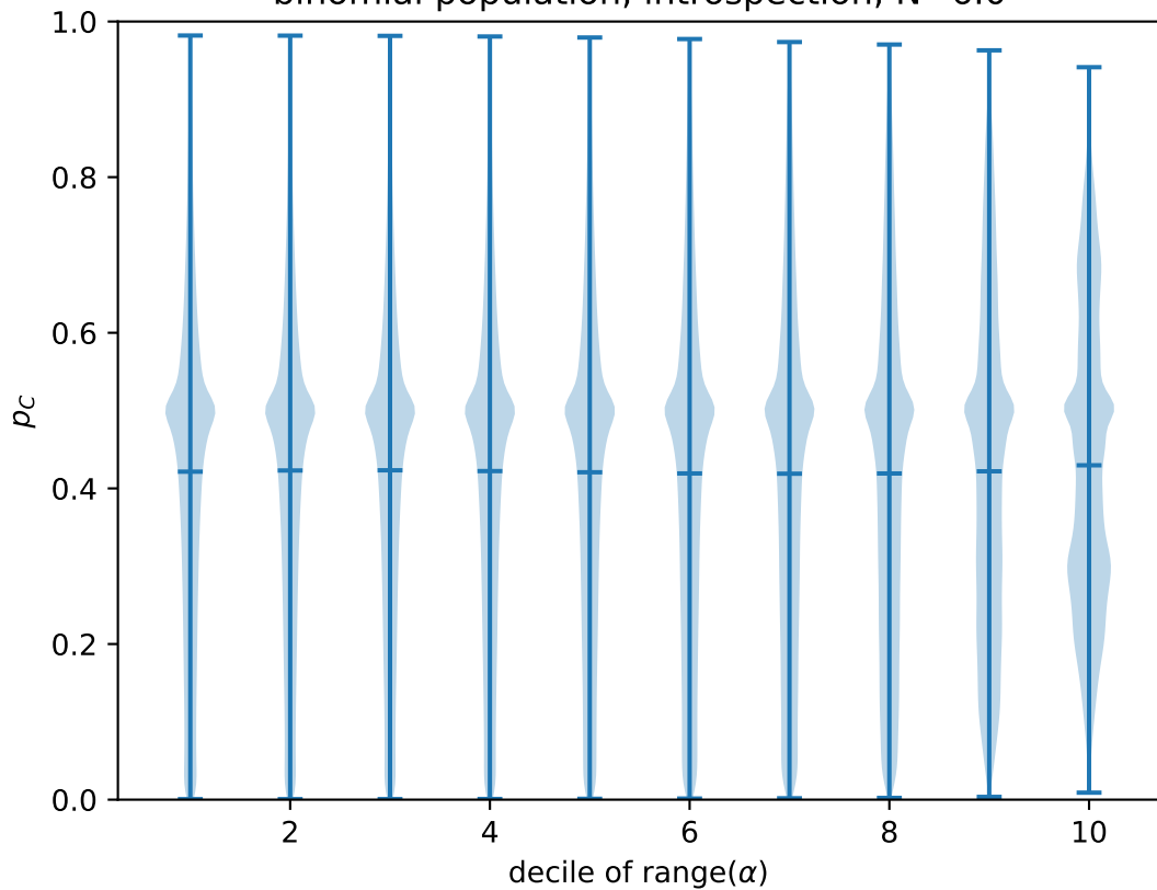
binomial population, introspection, N=6.0
