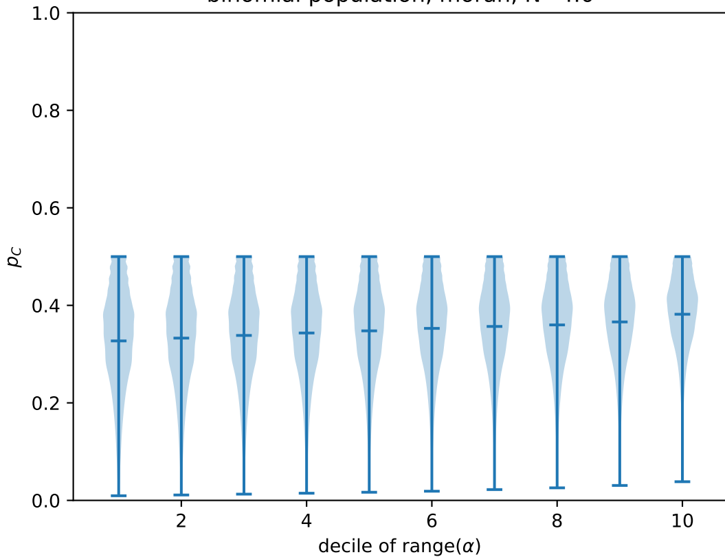
binomial population, moran, N=4.0
