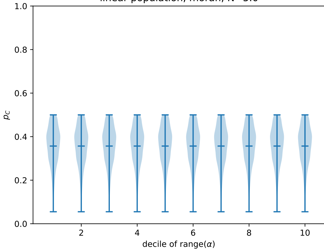
linear population, moran, N=5.0
