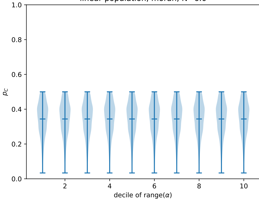
linear population, moran, N=6.0
