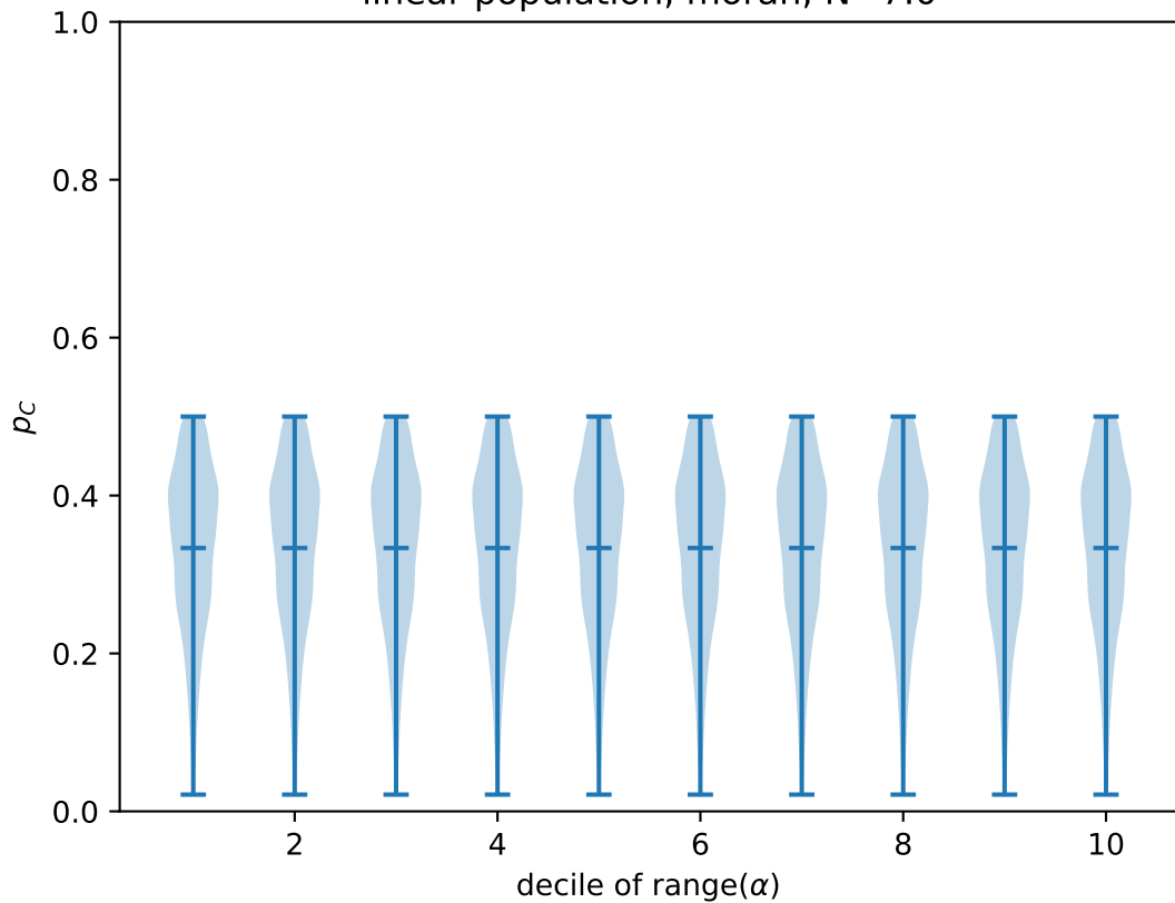
linear population, moran, N=7.0
