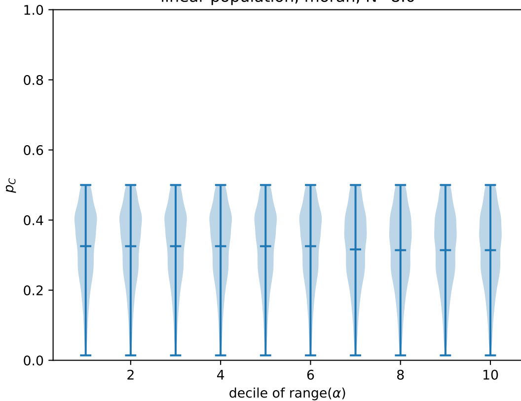
linear population, moran, N=8.0
