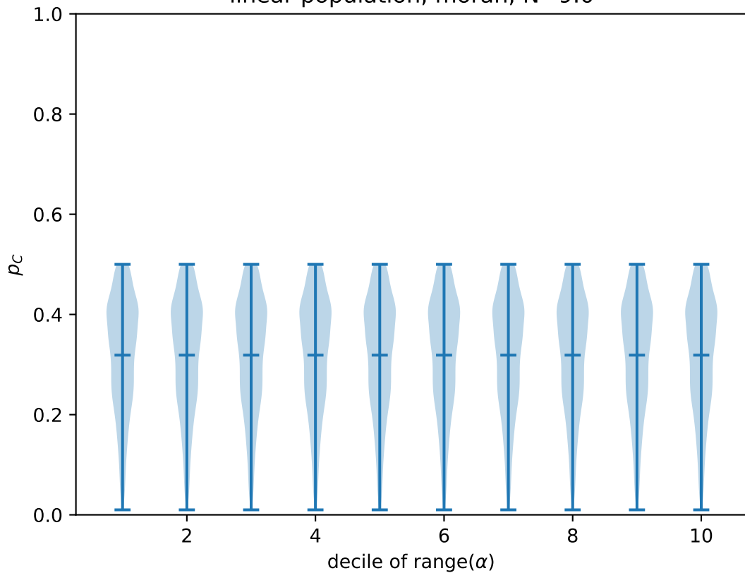
linear population, moran, N=9.0
