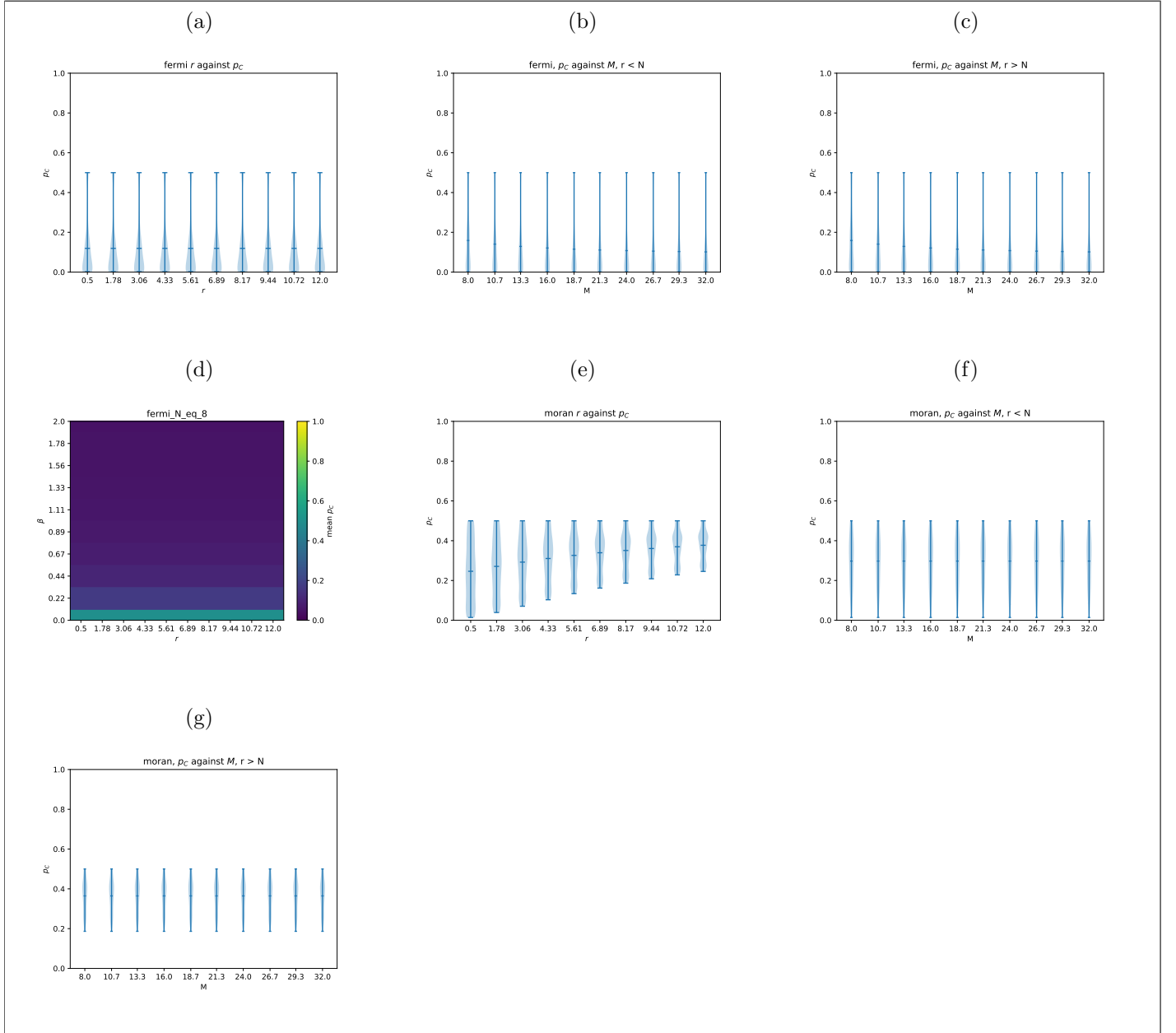
Figure 2: (a): The distribution of p_C in Fermi imitation dynamics for different values of r . Since Fermi imitation dynamics is invariant under the value of r , this distribution does not change, and for all values of r it admits a maximum value of p_C below the neutral-drift baseline p_C = \frac{1}{2} . (b) & (c): The distribution of p_C for Fermi imitation dynamics for different sizes of contribution. The greater the value of M , the greater the size of each player's contribution. (b) shows when r < N , and (c) shows r > N . (d): A heatmap of \text{mean}(p_C) for values of r and \beta for Fermi imitation dynamics. We see that there is a negative correlation between \beta and p_C . (e - g): The equivalent of (a - c) for the Moran process. (f): The distribution of difference in p_C between Fermi imitation dynamics and the Moran process for different combinations of shared parameters.
