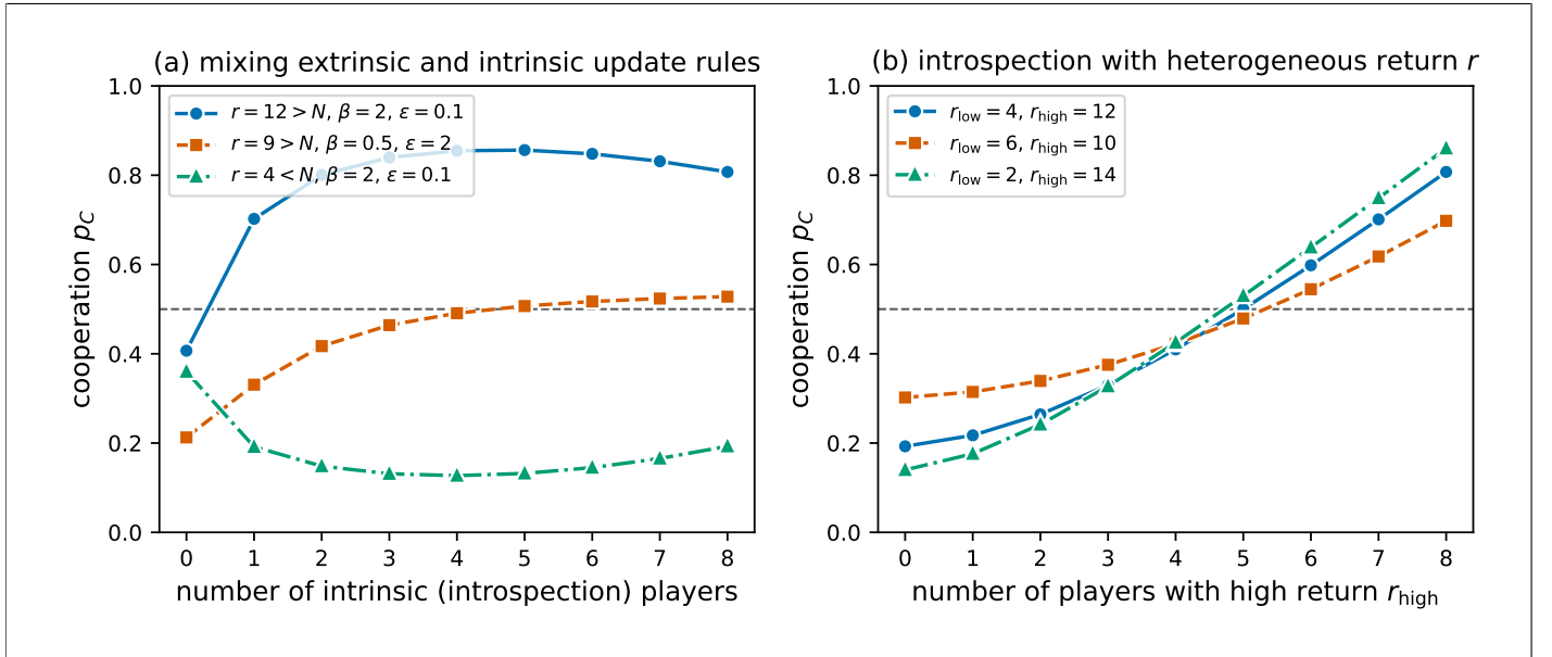
Figure 5: Heterogeneous update rules and heterogeneous returns. Both panels are computed exactly from the steady state of the corresponding transition matrix, with N = 8 , a linear contribution profile of scale M = 16 , and mutation \mu = 0.05 ; the dashed line marks the neutral-drift baseline p_C = \frac{1}{2} . (a) A population that mixes Moran (extrinsic) and introspection (intrinsic) players, against the number of introspection players: with r > N the population can exceed the baseline, but the number of intrinsic players required grows as the extrinsic selection intensity \varepsilon increases or the choice intensity \beta falls; with r < N the intrinsic players instead suppress cooperation. (b) Introspection dynamics with a heterogeneous return, against the number of players receiving the high return r_{\text{high}} ; cooperation crosses the ceiling once enough players sit above the threshold r = N .
