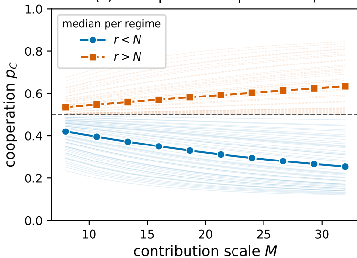
(c) introspection responds to \alpha_i
