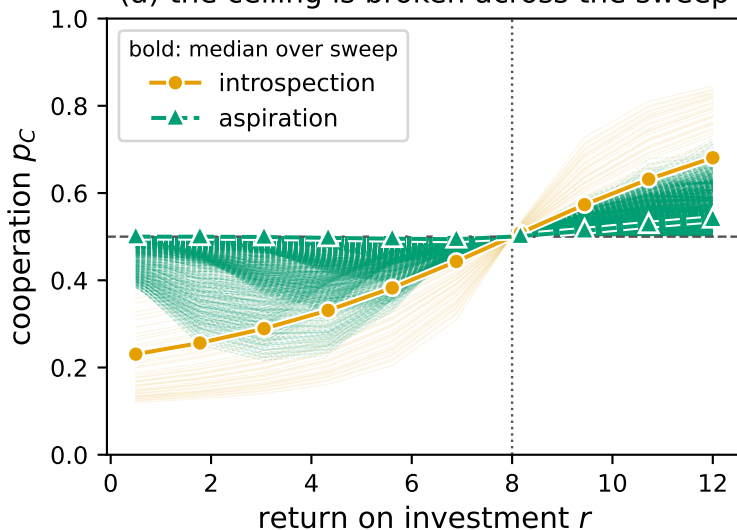
(a) the ceiling is broken across the sweep
