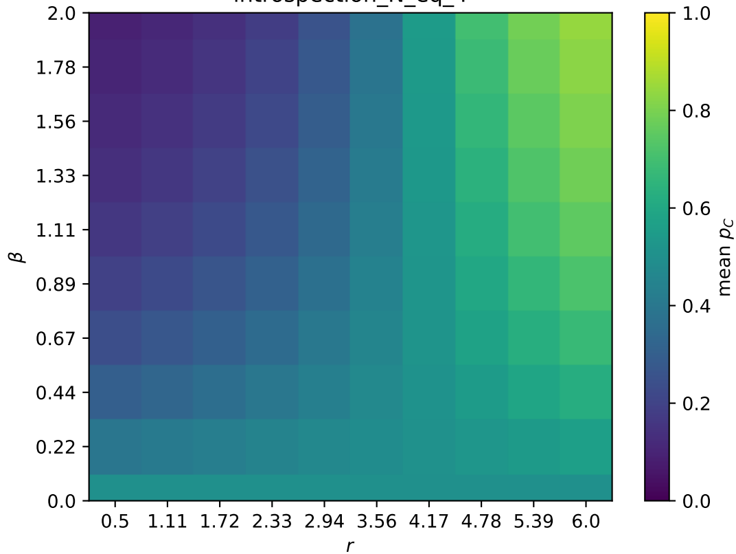
introspection_N_eq_4
