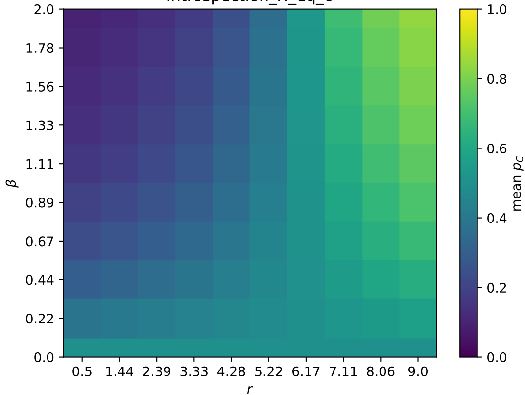
introspection_N_eq_6
