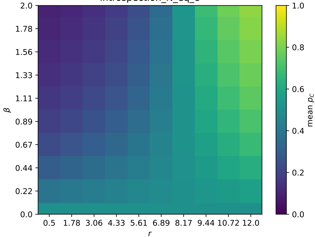
introspection_N_eq_8
