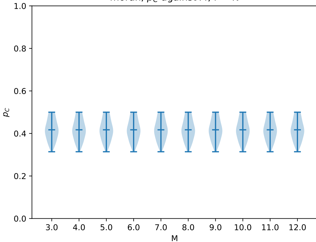
moran, p_c against M , r > N
