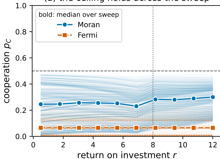
(a) the ceiling holds across the sweep
