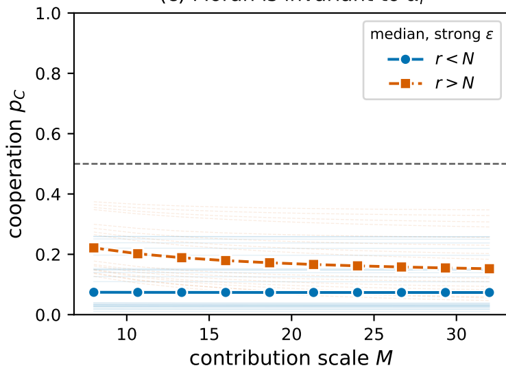
(c) Moran is invariant to \alpha_i
