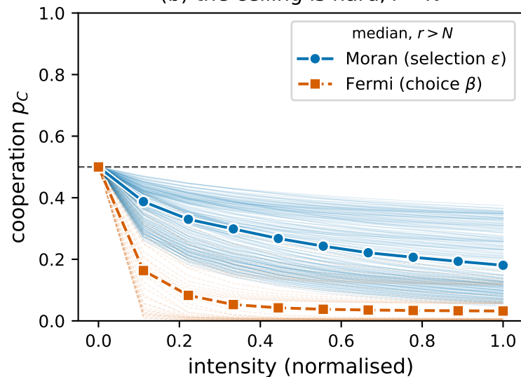
(b) the ceiling is hard, r > N
