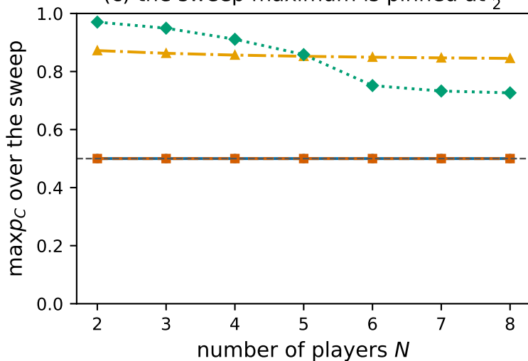
(c) the sweep maximum is pinned at \frac{1}{2}
