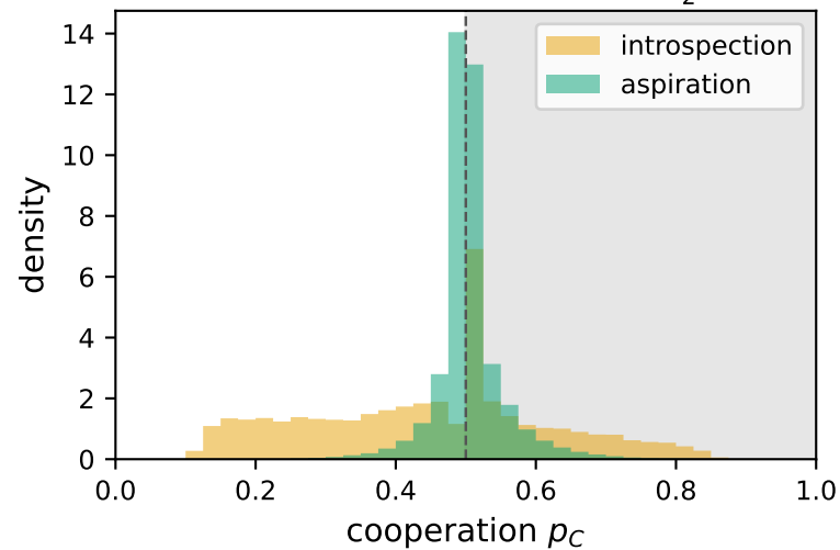
(b) intrinsic dynamics cross \frac{1}{2}
