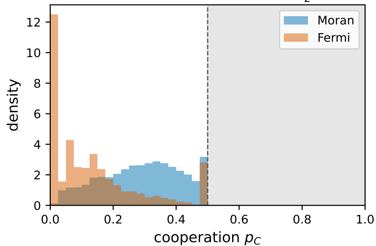
(a) purely extrinsic: all p_C \leq \frac{1}{2}
