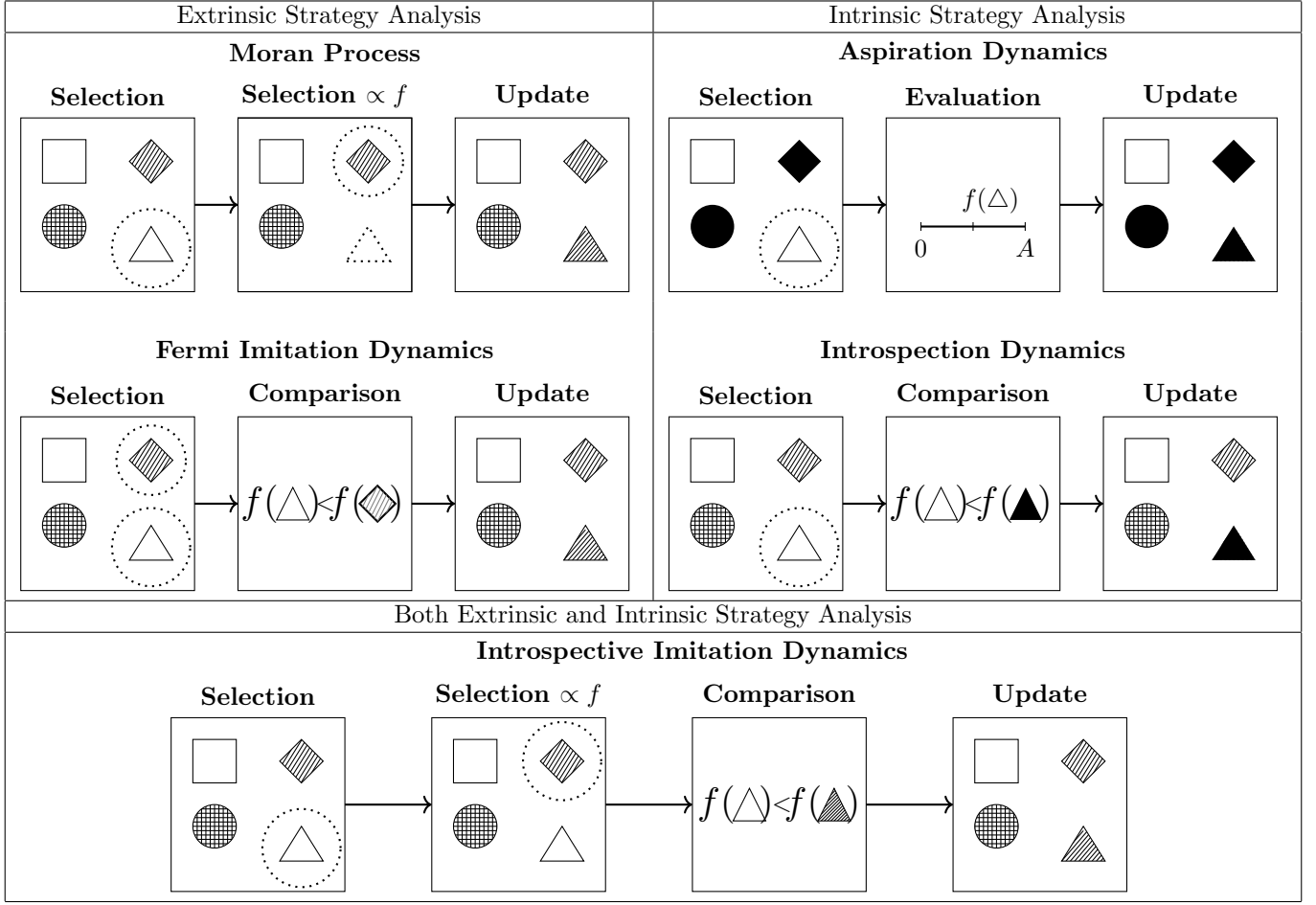
Figure 18: A comparison of different population dynamics. We assume in all cases that the triangle is chosen for replacement with a probability \frac{1}{N} and the diamond is chosen with a varying probability depending on the process. In the case of Introspection dynamics, we assume that the strategy represented by the shape being filled in is chosen with probability \frac{1}{k-1} , and for aspiration dynamics there is only one other strategy to accept.
