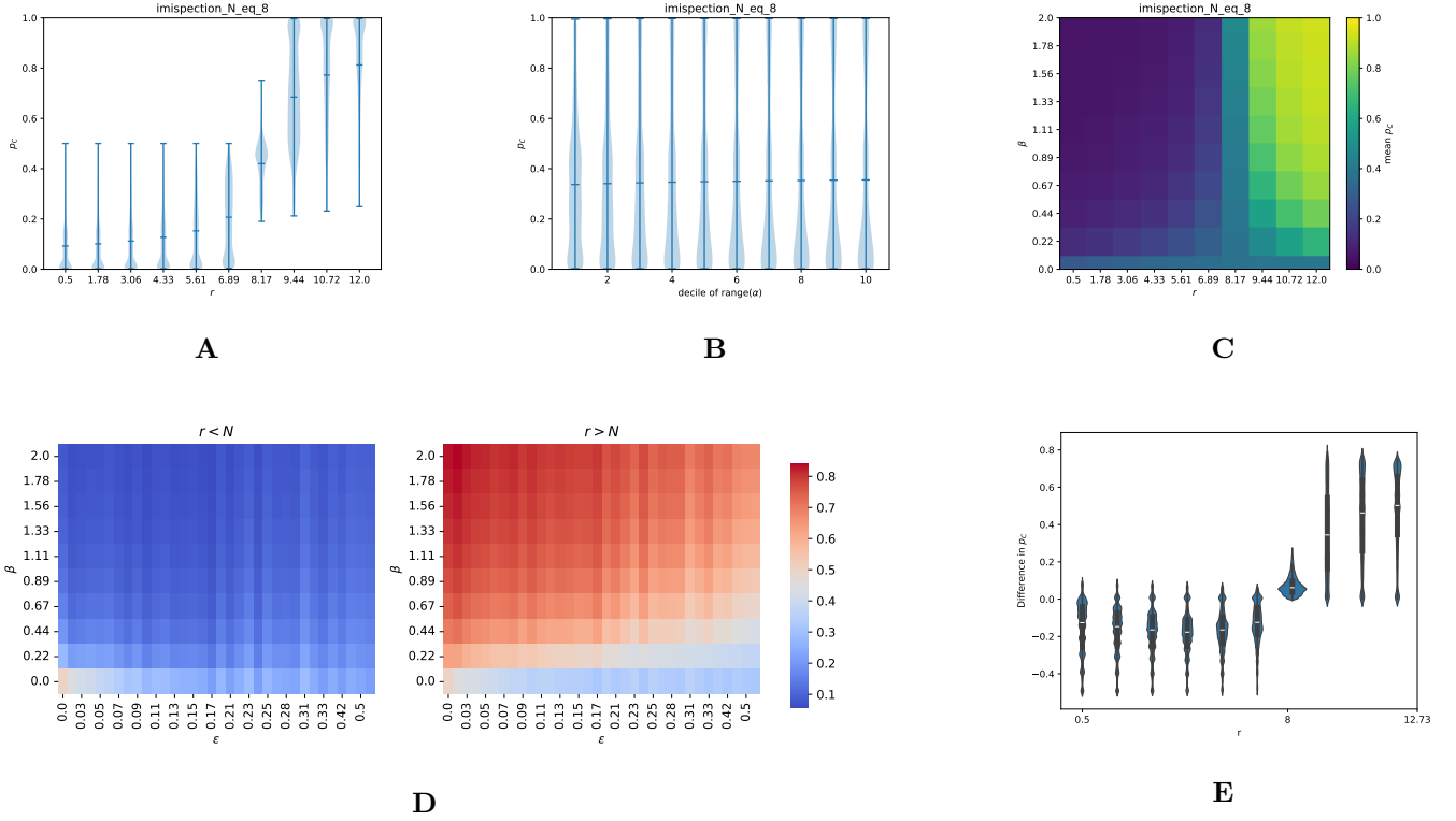
Figure 16: A: the distribution of p_C in introspective imitation dynamics for various values of r . B: the distribution of p_C in introspective imitation dynamics for various levels of heterogeneity. The greater the value of range( \alpha ), the greater the contribution heterogeneity. C: A heatmap of mean( p_C ) in introspective imitation dynamics for varying r and \beta . We see a threshold for the effect of a stronger choice intensity at r = N . D: A heatmap of the effect of both selection and choice intensity on mean( p_C ) for r > N and r < N . E: The difference in p_C between introspective imitation dynamics and the Moran process for populations with shared parameters, specifically for different values of r .
