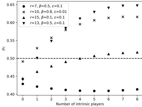
Figure 9: A: p_C in various parameter combinations at N = 8 , varying the number of players using an intrinsic population dynamic. B: for various parameter combinations, the mean value over numerous simulations of an 8 player population playing introspective imitation dynamics converging to the theoretic p_C .
