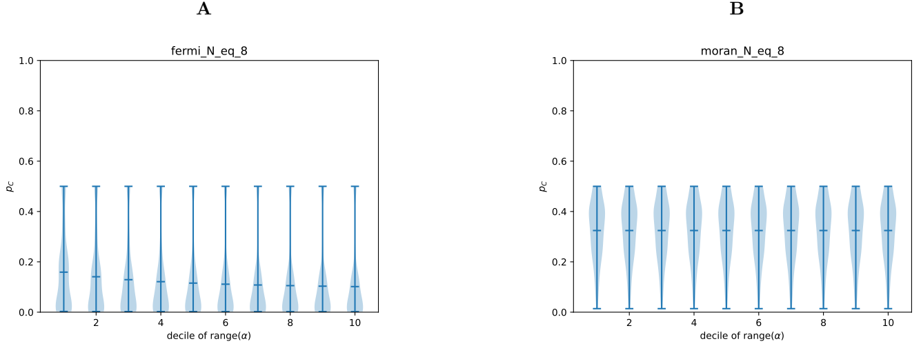
Figure 5: The distribution of p_C for each dynamic for different levels of heterogeneity in contribution. The greater the decile of \text{range}(\alpha_i) , the greater the heterogeneity in contribution. A shows fermi imitation dynamics, B shows the Moran process.
