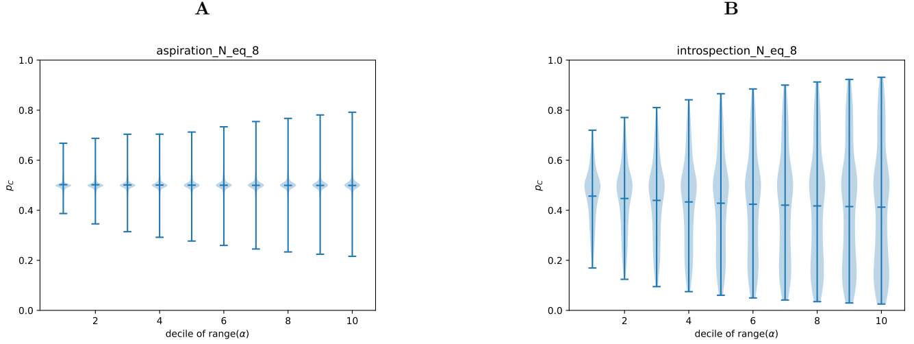
Figure 8: The distribution of p_C for each dynamic for different levels of heterogeneity in contribution. The greater the decile of \text{range}(\alpha_i) , the greater the heterogeneity in contribution. A shows aspiration dynamics, B shows introspection dynamics.
