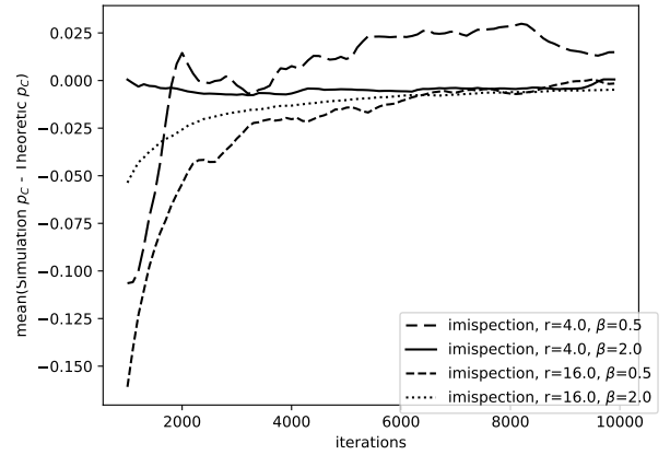
Figure 9: A: p_C in various parameter combinations at N = 8 , varying the number of players using an intrinsic population dynamic. B: for various parameter combinations, the mean value over numerous simulations of an 8 player population playing introspective imitation dynamics converging to the theoretic p_C .
