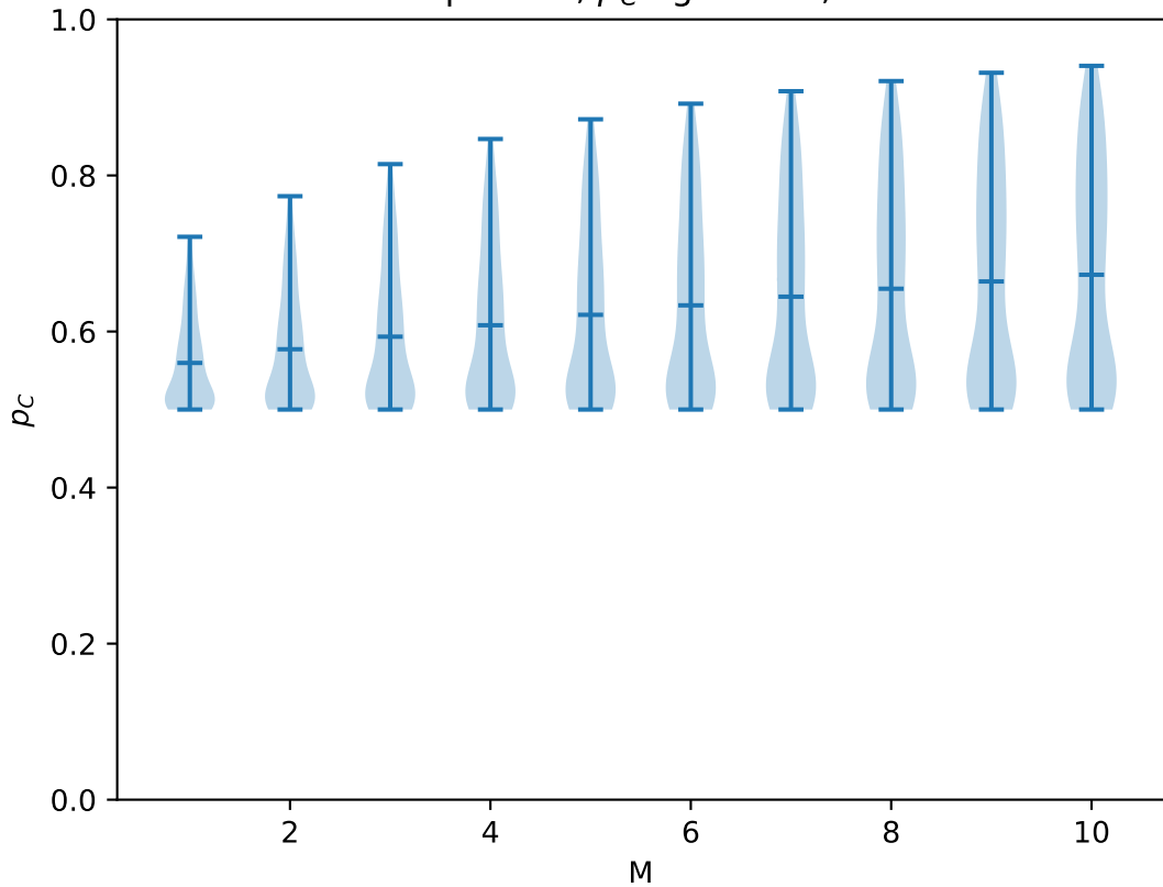
introspection, p_C against M , r > N
