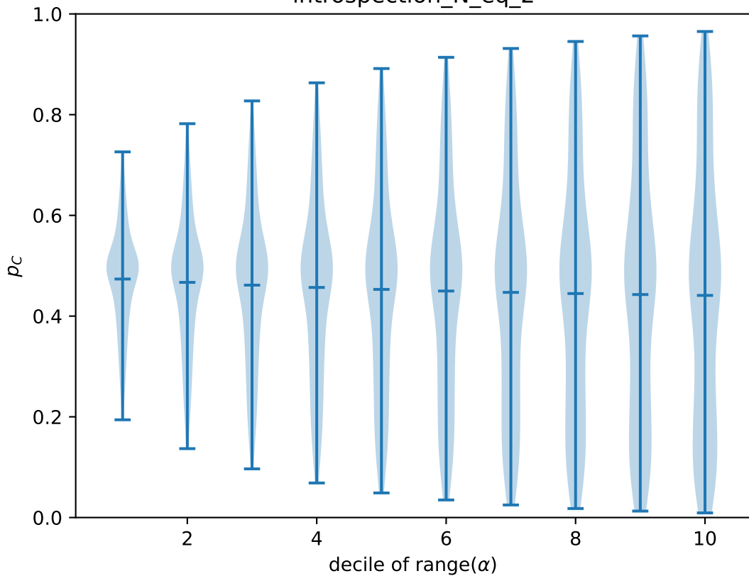
introspection_N_eq_2
