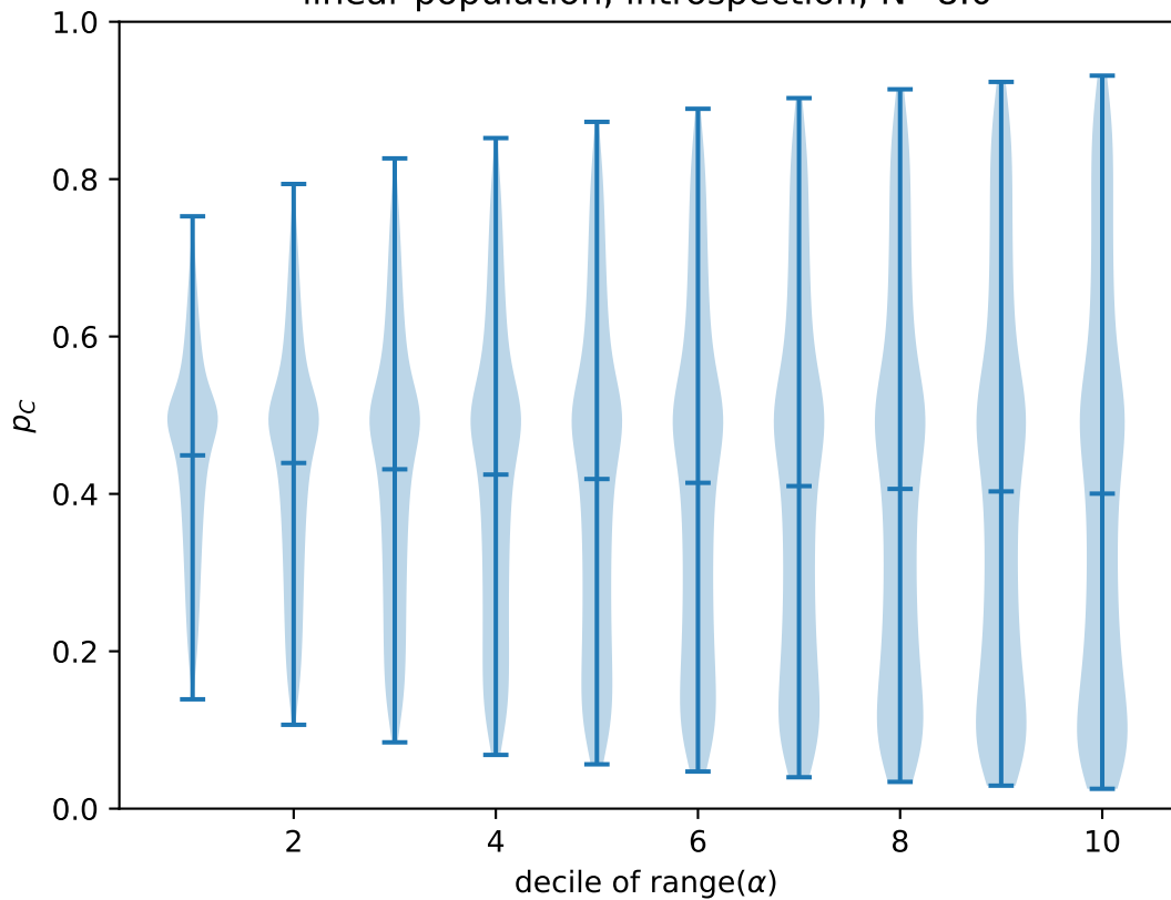
linear population, introspection, N=8.0
