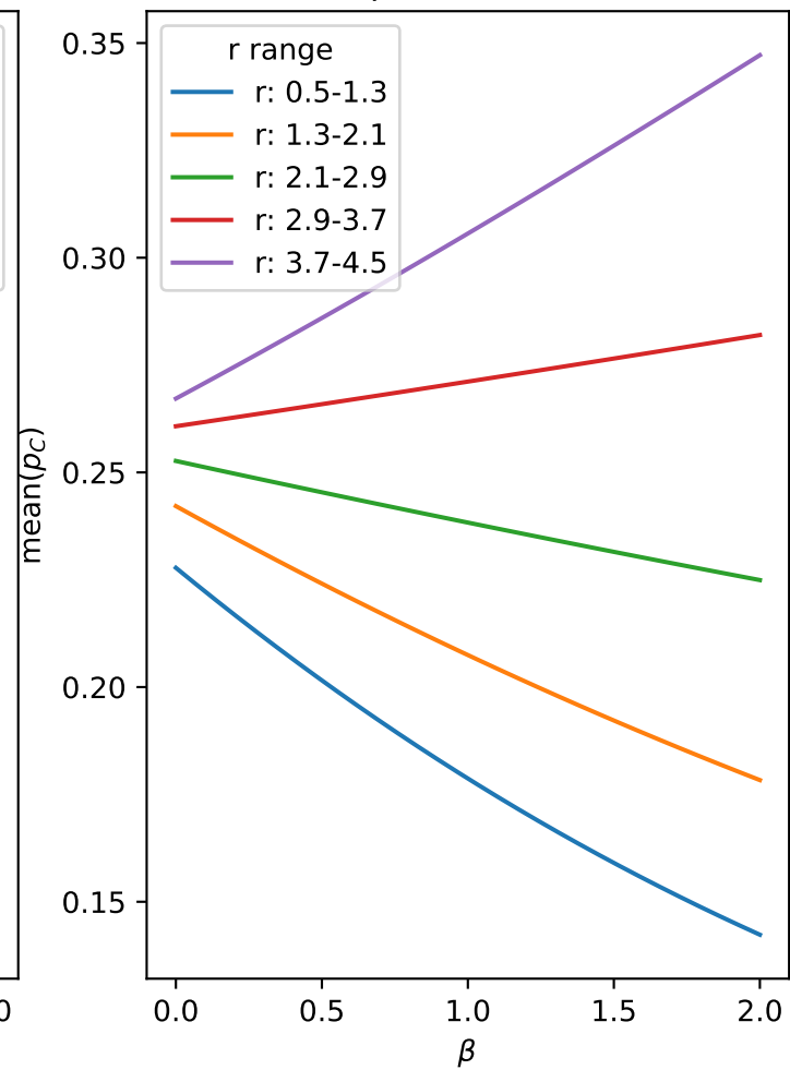
Introspective Imitation
