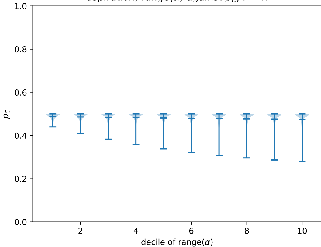
aspiration, range( \alpha ) against p_C , r < N
