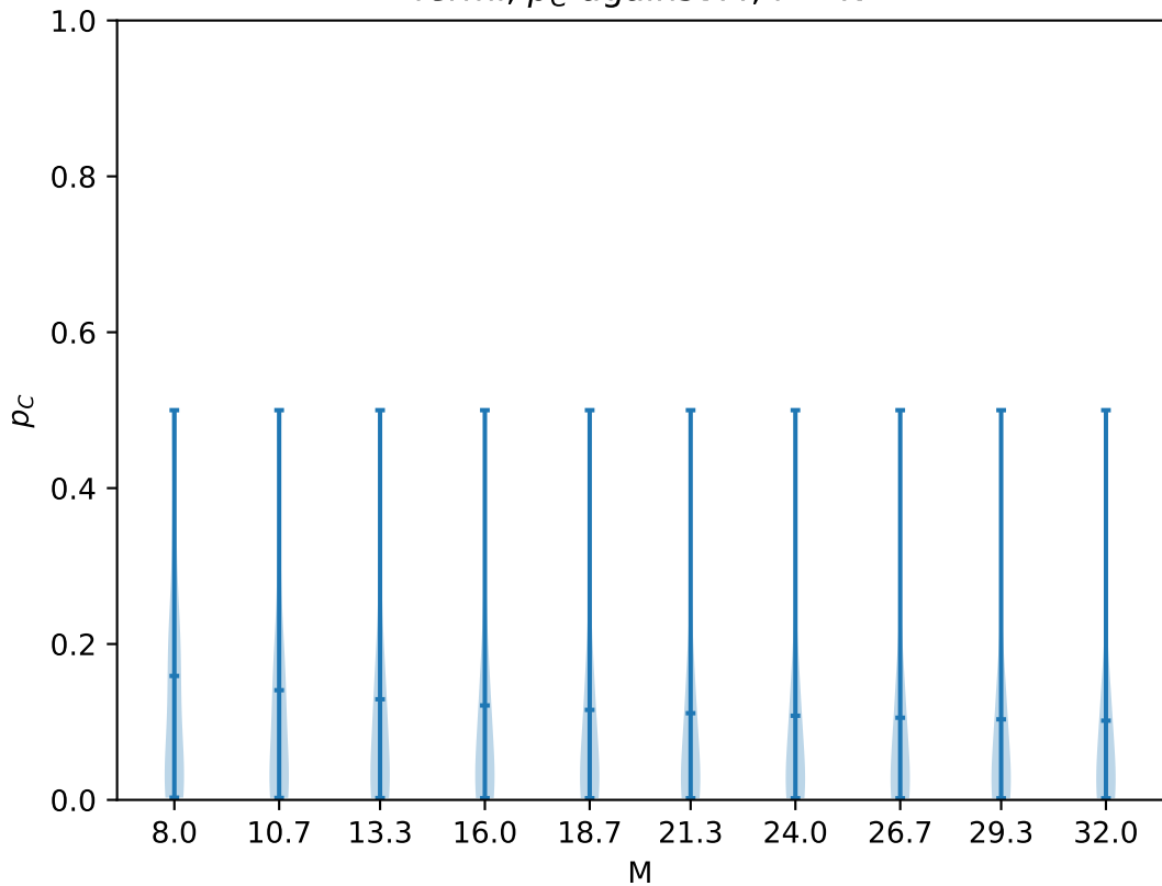
fermi, p_C against M , r > N
