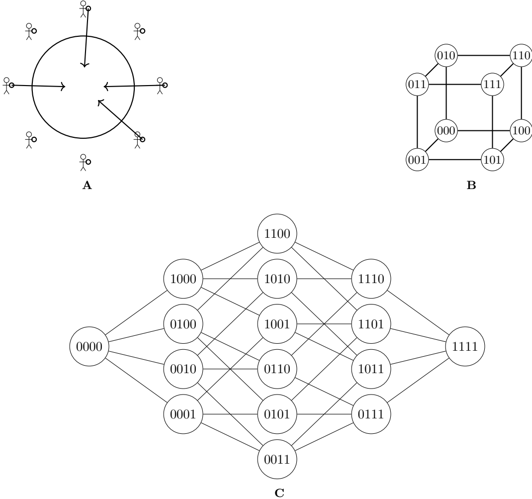
Figure 1: A : The public goods game with 8 players. Here 4 players contribute. B : The graph of a 3-player game with 2 actions under a birth-death process. This is closely related to the hypercube of dimension 3. C : The graph of a 4-player game with 2 actions under a birth-death process. This representation shows how one player changes action at a given time.
