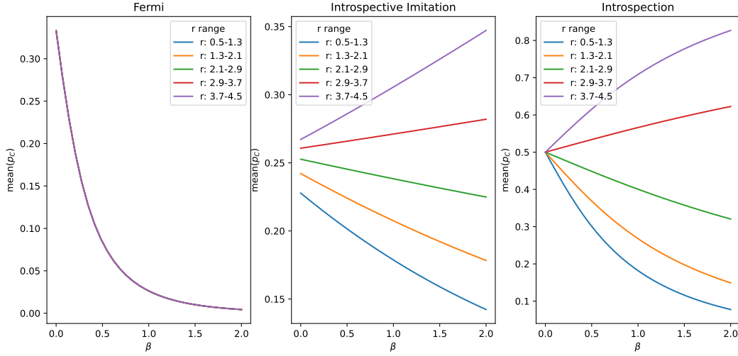
Figure 9: p_C as a function of choice intensity \beta and multiplier r , comparing extrinsic and intrinsic dynamics.
