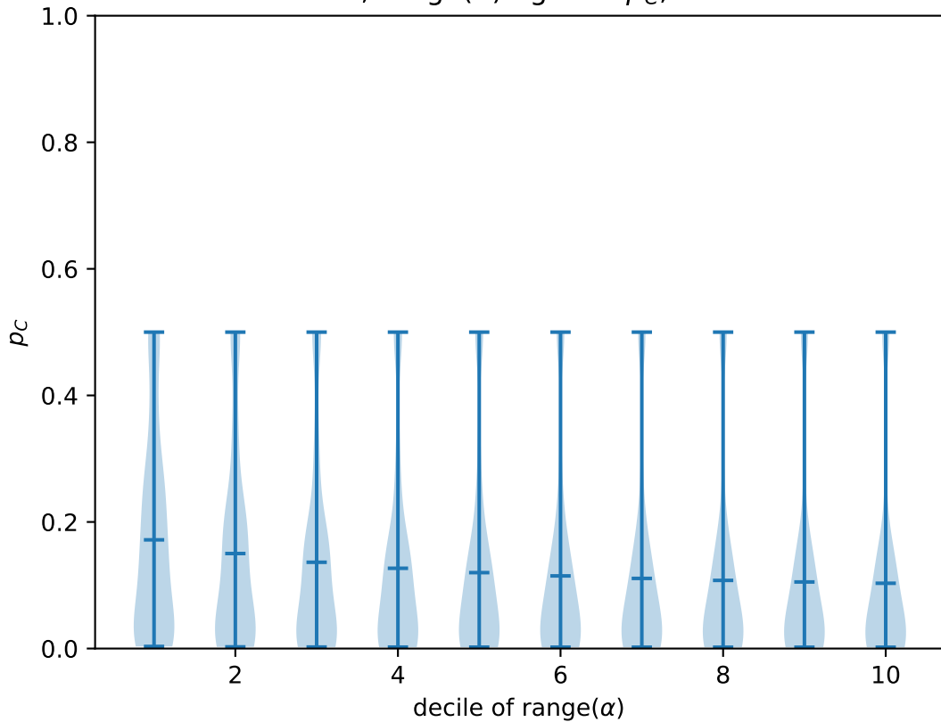
fermi, range( \alpha ) against p_C , r < N
