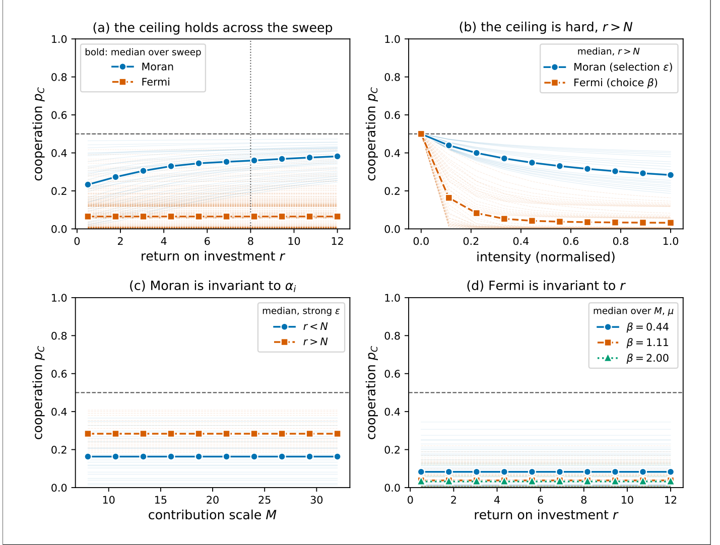
Figure 2: The cooperation ceiling under purely extrinsic dynamics. Throughout, N = 8 , a linear contribution profile, and mutation \mu = 0.05 ; the dashed line marks the neutral-drift baseline p_C = \frac{1}{2} and, in (a), the dotted line marks r = N . Faint curves show the p_C trajectory of every parameter set in the sweep (coincident trajectories are drawn once), and the bold curves their median taken over all parameter sets. (a) Cooperation p_C against the return r : the Moran process rises with r but never exceeds \frac{1}{2} , and Fermi imitation dynamics stays well below it. (b) With r > N , p_C against the normalised selection intensity \varepsilon (Moran) and choice intensity \beta (Fermi); neither exceeds \frac{1}{2} , reaching it only as the intensity vanishes. (c) The Moran process is invariant to the contribution scale M , as derived in Equation (7). (d) Fermi imitation dynamics is invariant to the return r , as derived in Equation (6).
