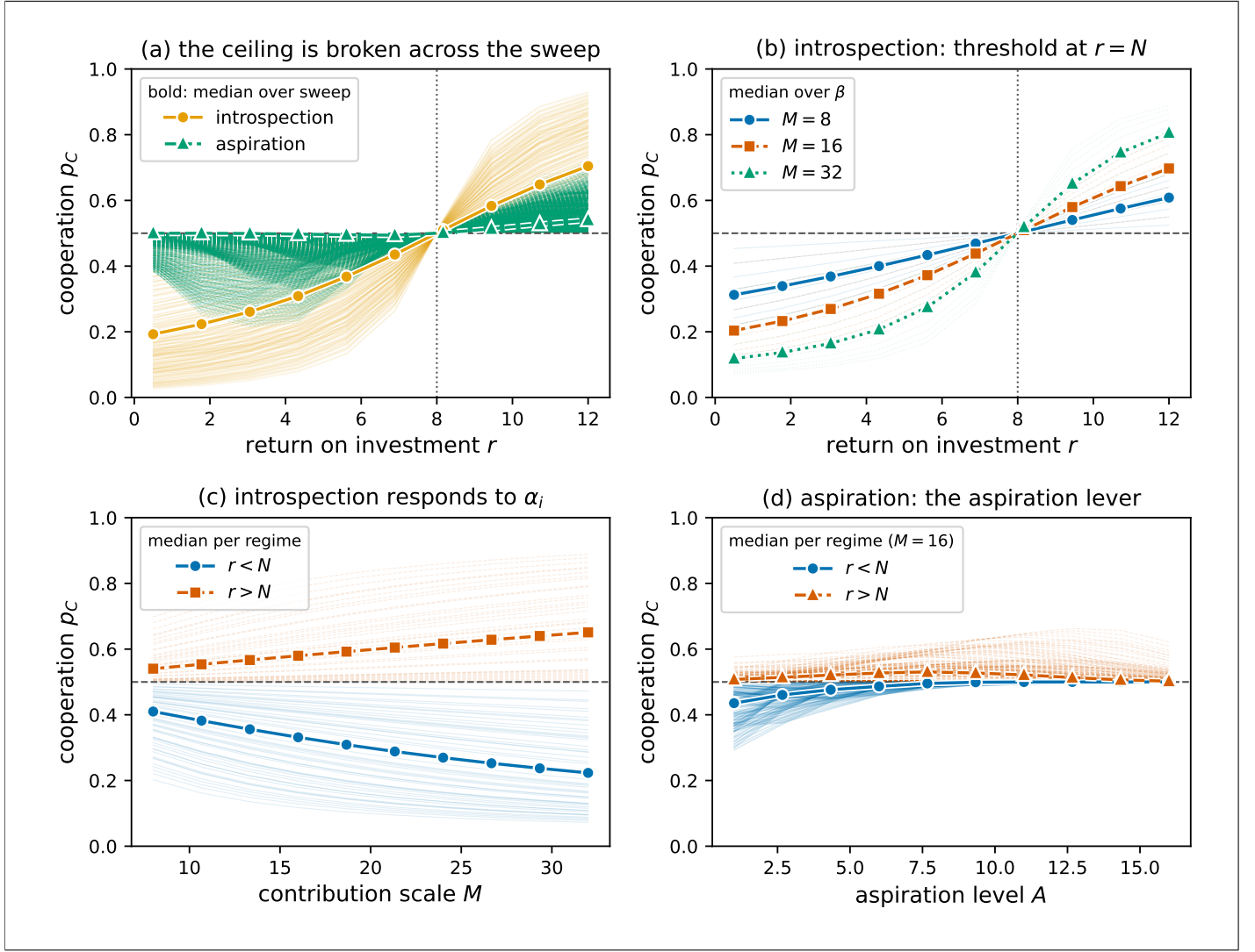
Figure 3: Intrinsic dynamics exceed the cooperation ceiling. Same population as Figure 2; faint curves show the p_C trajectory of every parameter set in the sweep (coincident trajectories are drawn once), and the bold curves their median taken over all parameter sets, with the dashed line at p_C = \frac{1}{2} and the dotted line at r = N . (a) Cooperation p_C against the return r for introspection and aspiration dynamics; both exceed \frac{1}{2} once r > N . (b) Introspection p_C against r at several contribution scales M , every curve crossing \frac{1}{2} exactly at r = N : the threshold is set by the sign of the counterfactual payoff difference \Delta(\pi_{I(a,b)}) in Equation (10). (c) Introspection p_C against M : it increases with the contribution scale when r > N and decreases when r < N . (d) Aspiration p_C against the aspiration level A at M = 16 .
