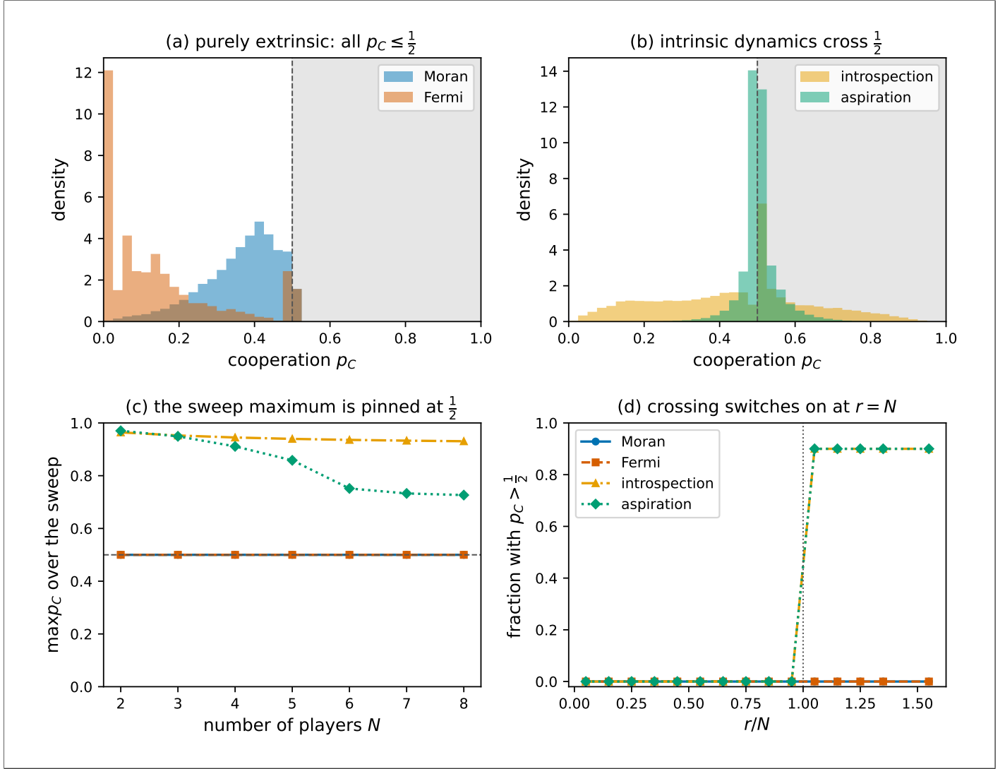
Figure 4: The cooperation ceiling across the entire sweep. Each panel pools every parameter combination with \mu > 0 . (a) The distribution of p_C for the purely extrinsic dynamics lies entirely at or below the neutral-drift baseline p_C = \frac{1}{2} (shaded region). (b) The intrinsic dynamics place mass above \frac{1}{2} . (c) The maximum p_C attained anywhere in the sweep, as a function of N : for the extrinsic dynamics it is pinned at exactly \frac{1}{2} at every N . (d) The fraction of parameter sets with p_C > \frac{1}{2} as a function of r/N : it is zero for the extrinsic dynamics at every return, and for the intrinsic dynamics switches on precisely at r = N .
