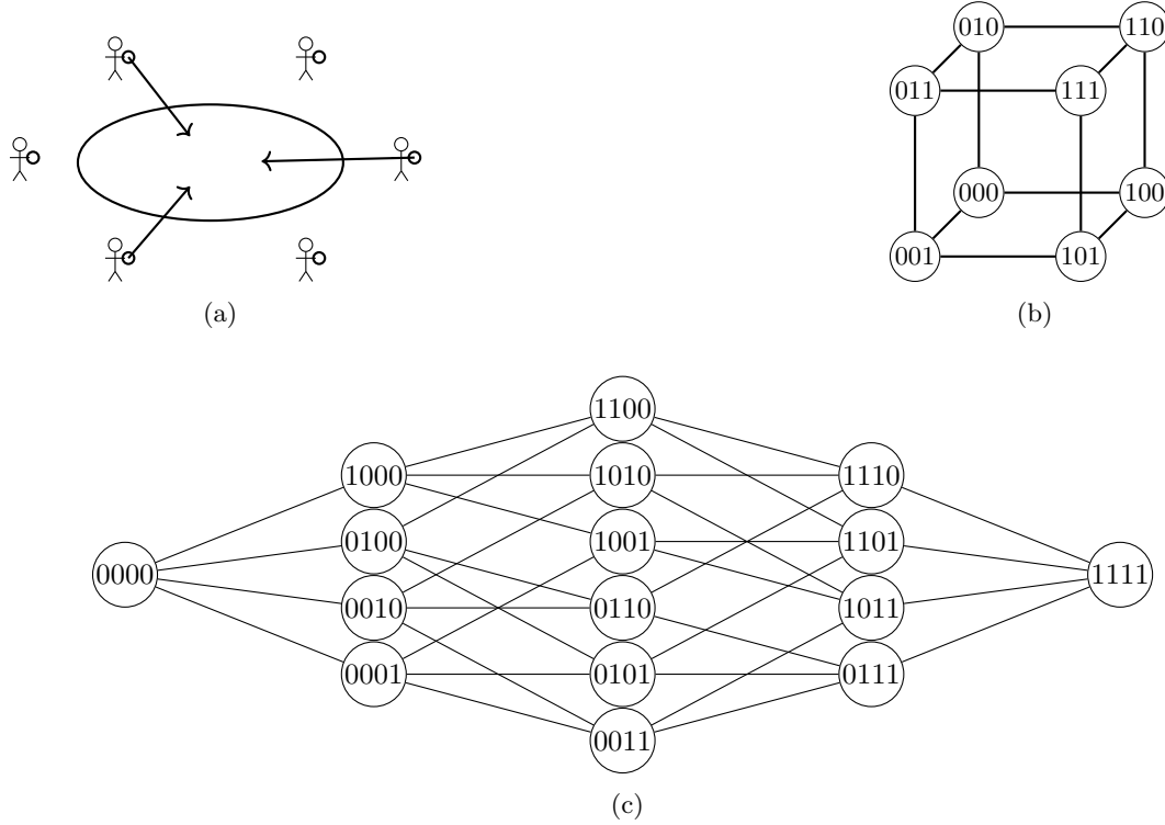
Figure 2: (a): The public goods game with 6 players. Here 3 players contribute. (b): The hypercube of dimension 3. This is closely related to the graph of a 3-player population dynamic. (c): The hypercube of dimension 4. This is closely related to the graph of a 4-player population dynamic.
