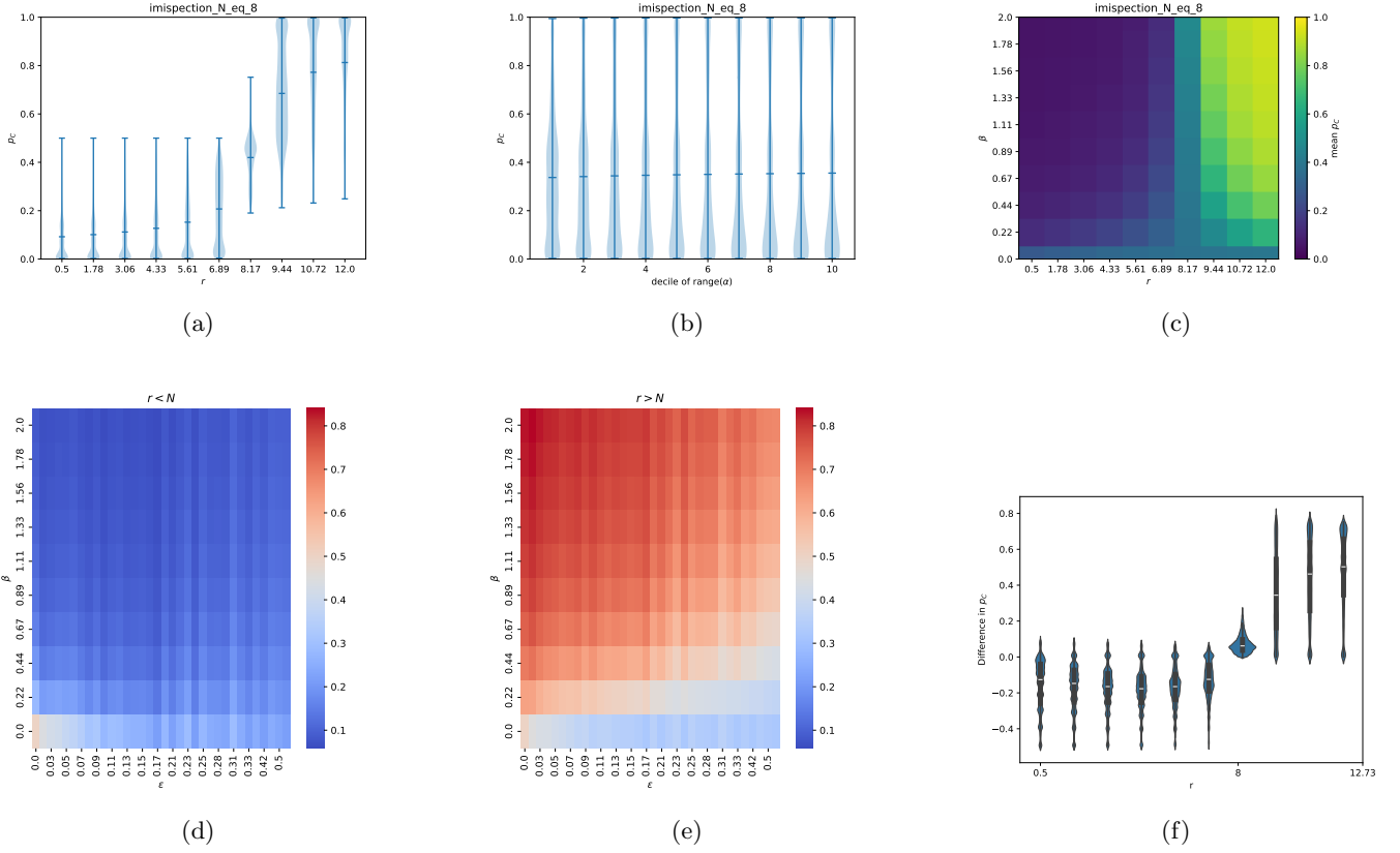
Figure 5: (a): the distribution of p_C in introspective imitation dynamics for various values of r . (b): the distribution of p_C in introspective imitation dynamics for various levels of heterogeneity. The greater the value of \text{range}(\alpha) , the greater the contribution heterogeneity. (c): A heatmap of \text{mean}(p_C) in introspective imitation dynamics for varying r and \beta . We see a threshold for the effect of a stronger choice intensity at r = N . (d),(e): Heatmaps of the effect of both selection and choice intensity on \text{mean}(p_C) for r > N and r < N . (f): The difference in p_C between introspective imitation dynamics and the Moran process for populations with shared parameters, specifically for different values of r .
