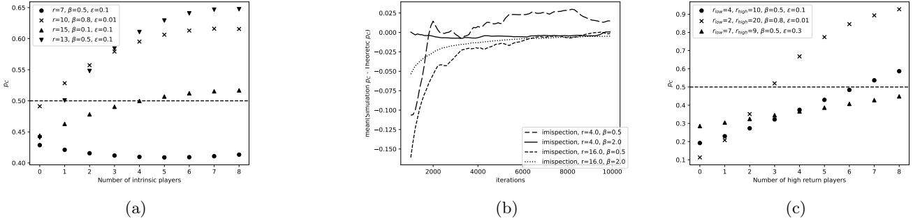
Figure 6: (a): p_C in various parameter combinations at N = 8 , varying the number of players using an intrinsic population dynamic. 0 intrinsic players gives the p_C of the Moran process, whereas 8 gives us the p_C in introspective imitation dynamics. We take a linear population with a maximum contribution of 8.
