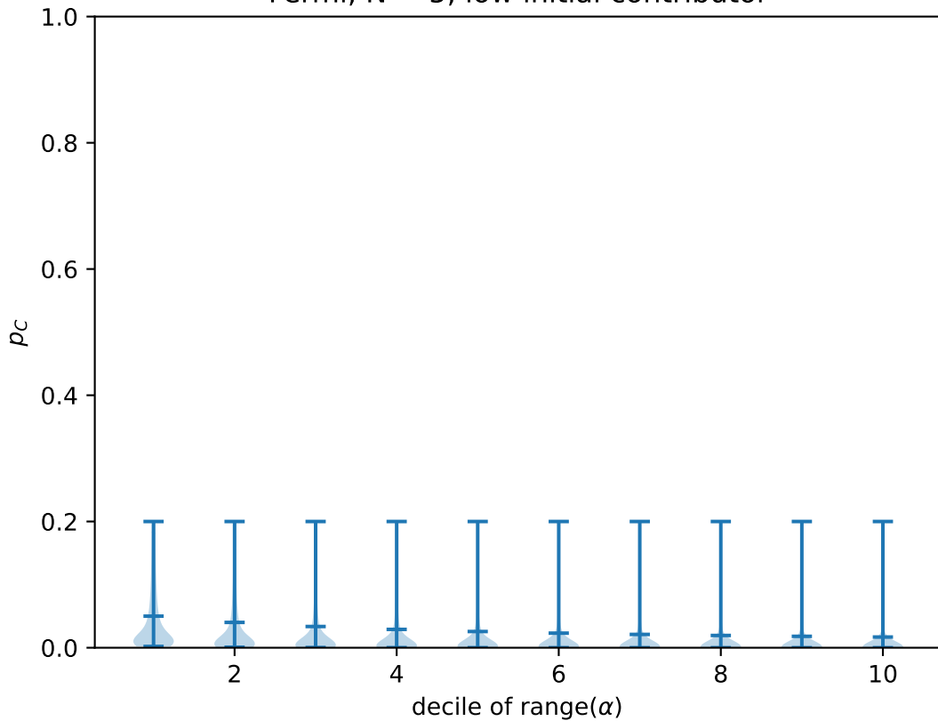
Fermi, N = 5 , low initial contributor
