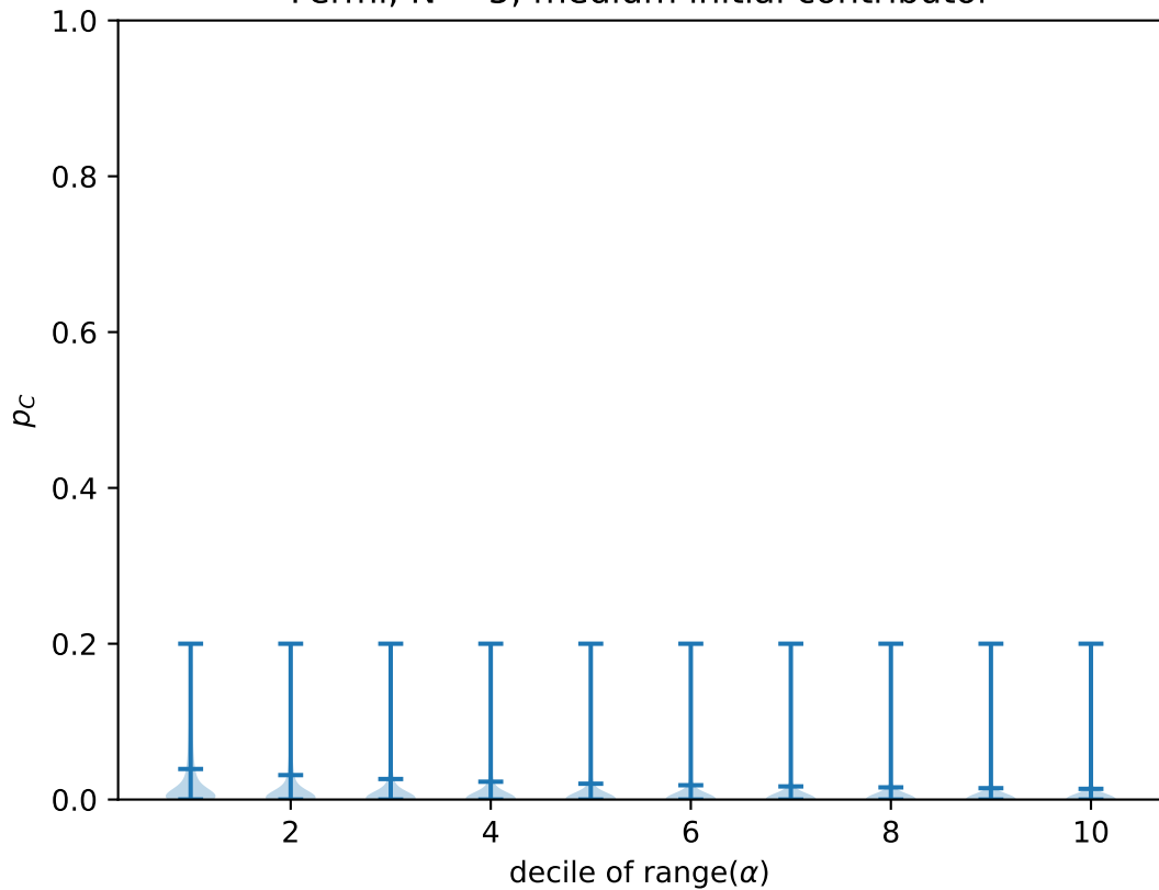
Fermi, N = 5 , medium initial contributor
