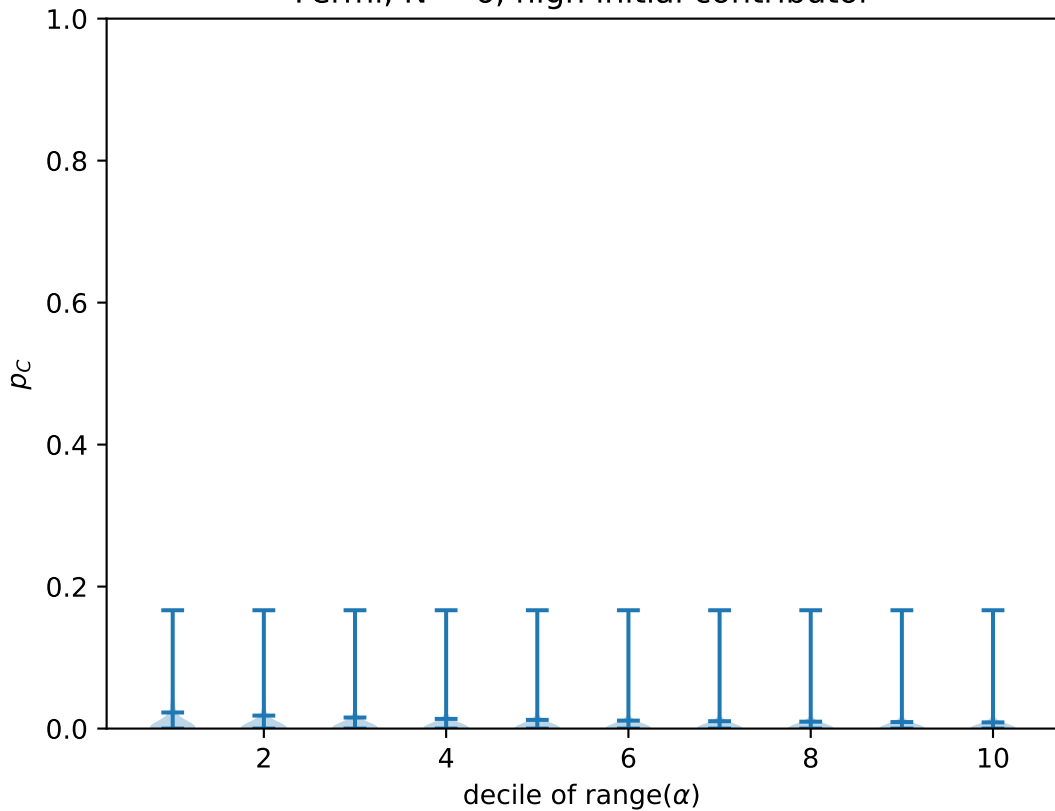
Fermi, N = 6 , high initial contributor
