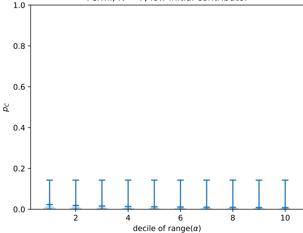
Fermi, N = 7 , low initial contributor
