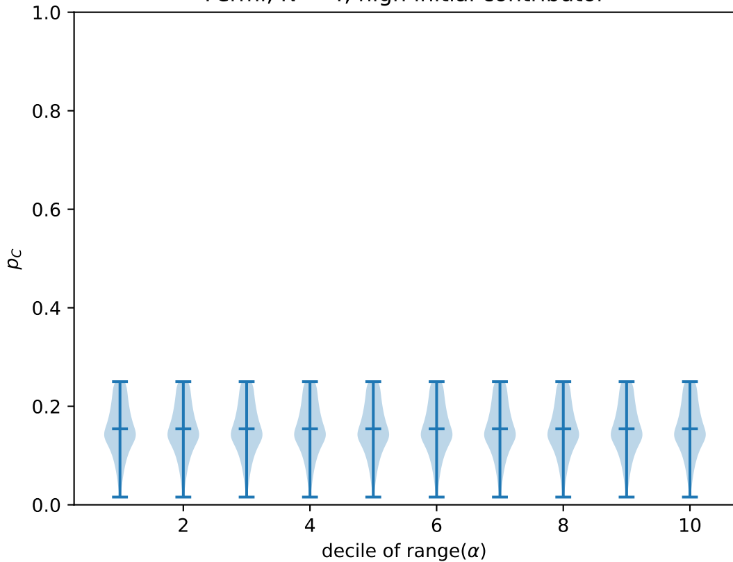
Fermi, N = 4 , high initial contributor
