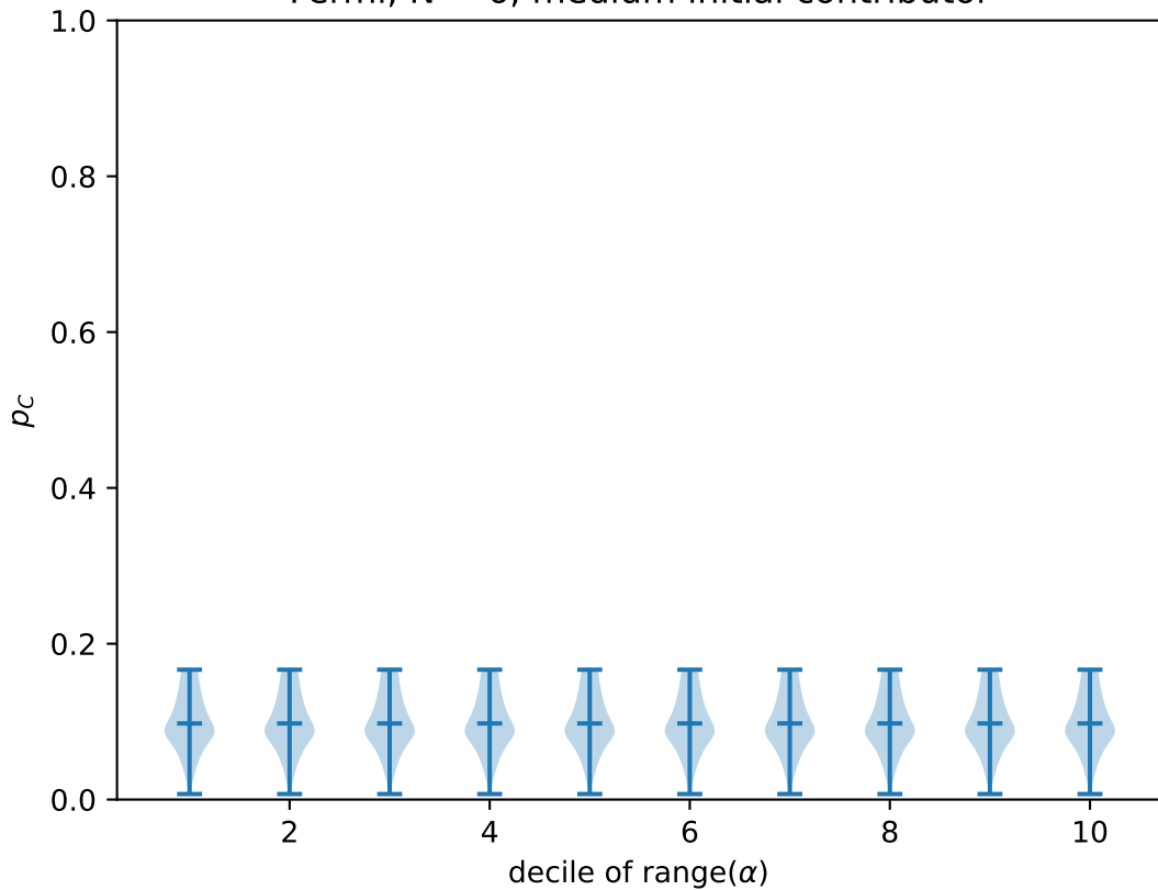
Fermi, N = 6 , medium initial contributor
